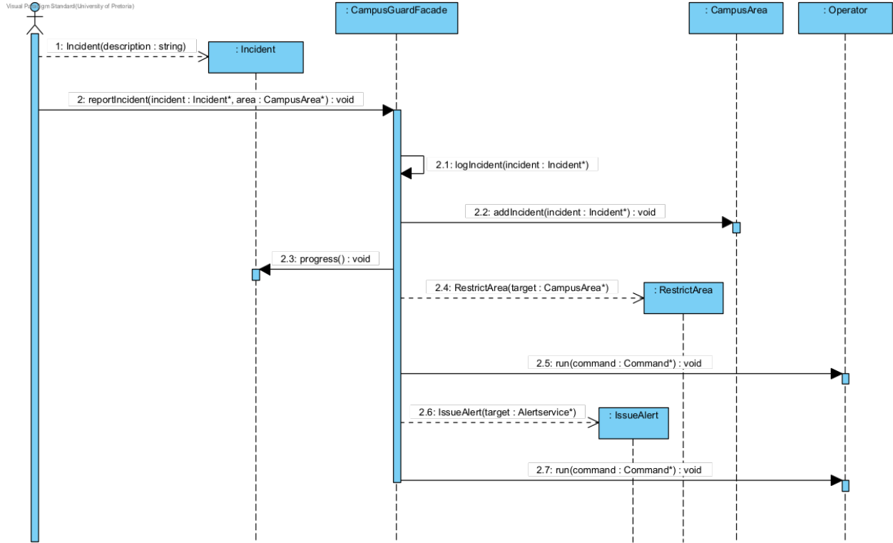
Figure 8: CampusGuardFacade reportIncident
