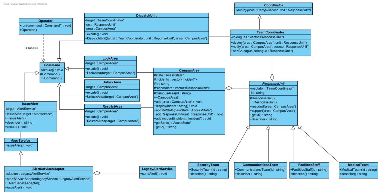
Figure 4: Command, Mediator and Adapter
