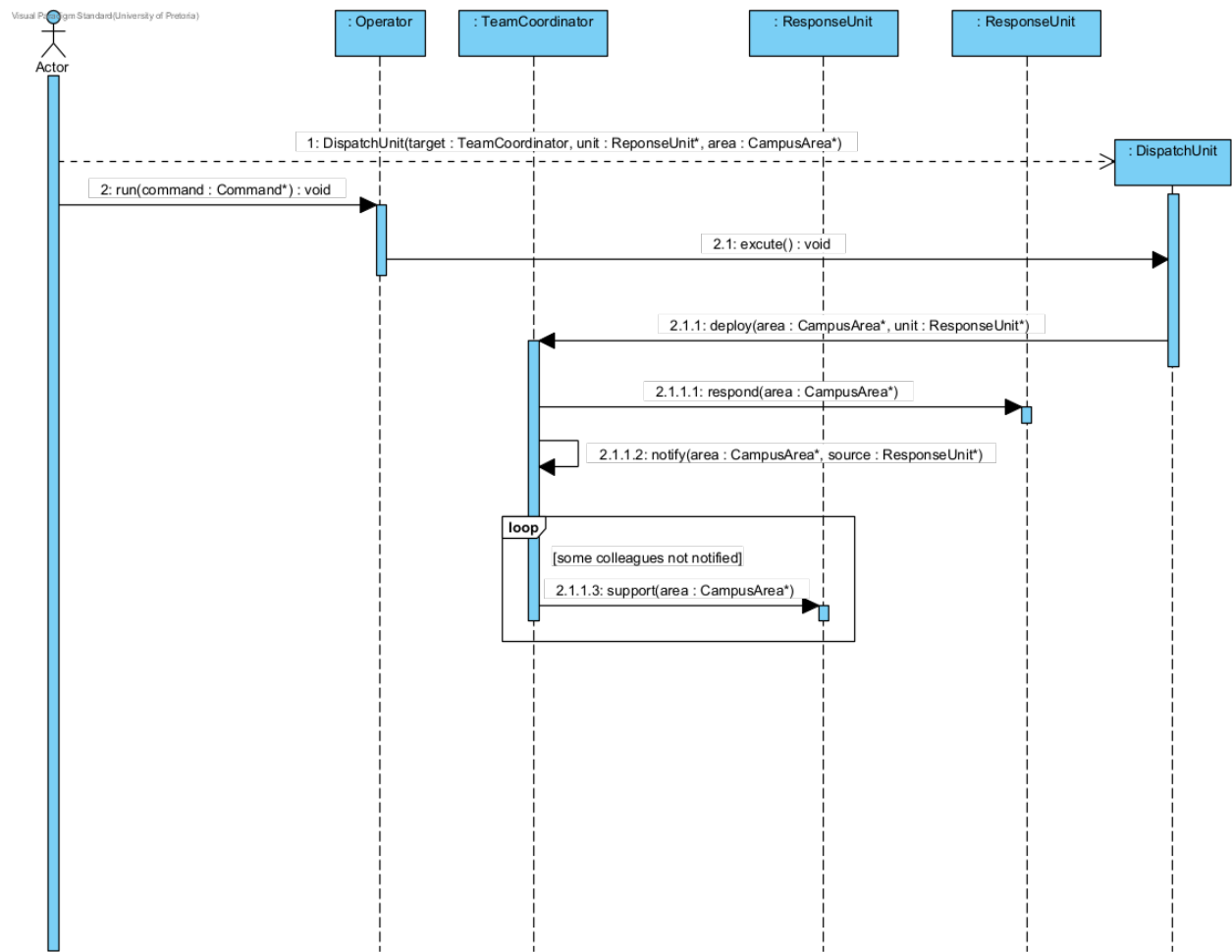
Figure 7: DispatchUnit through TeamCoordinator, then support from the other teams
