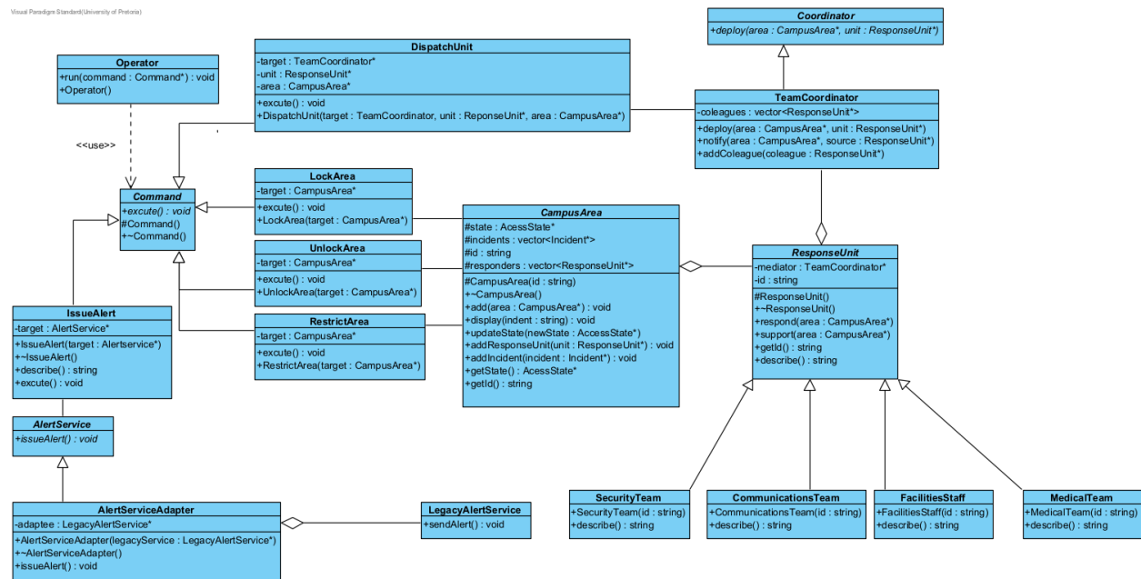
Figure 1: Command, Mediator and Adapter
