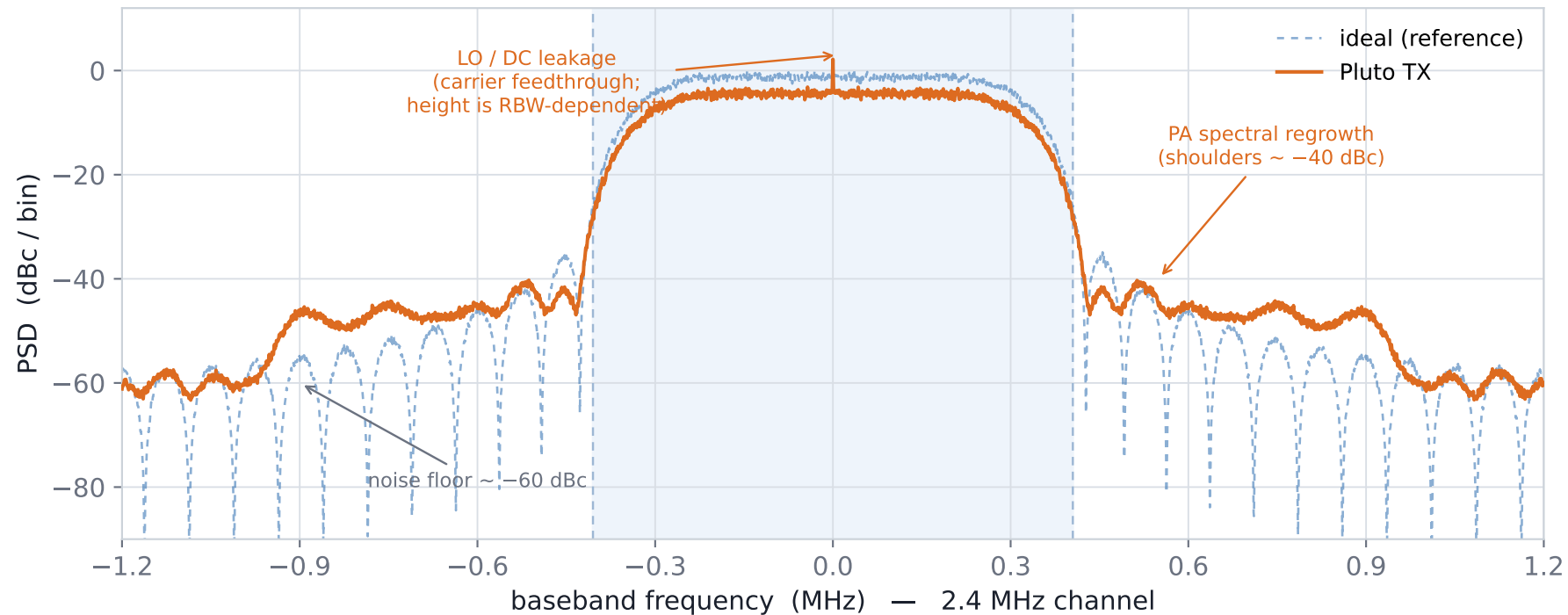
(b) ADALM-Pluto (AD9363 zero-IF) — same waveform, real front end
