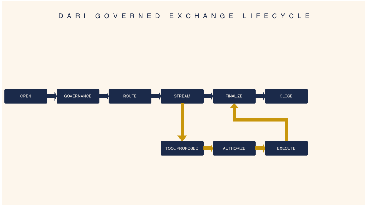
Figure 2: Conceptual protocol-design view of a Governed Exchange. Protected work advances through ordered authority gates; a model-generated tool proposal requires an independent authorization transition before execution. This figure specifies intended semantics, not measured implementation coverage.
