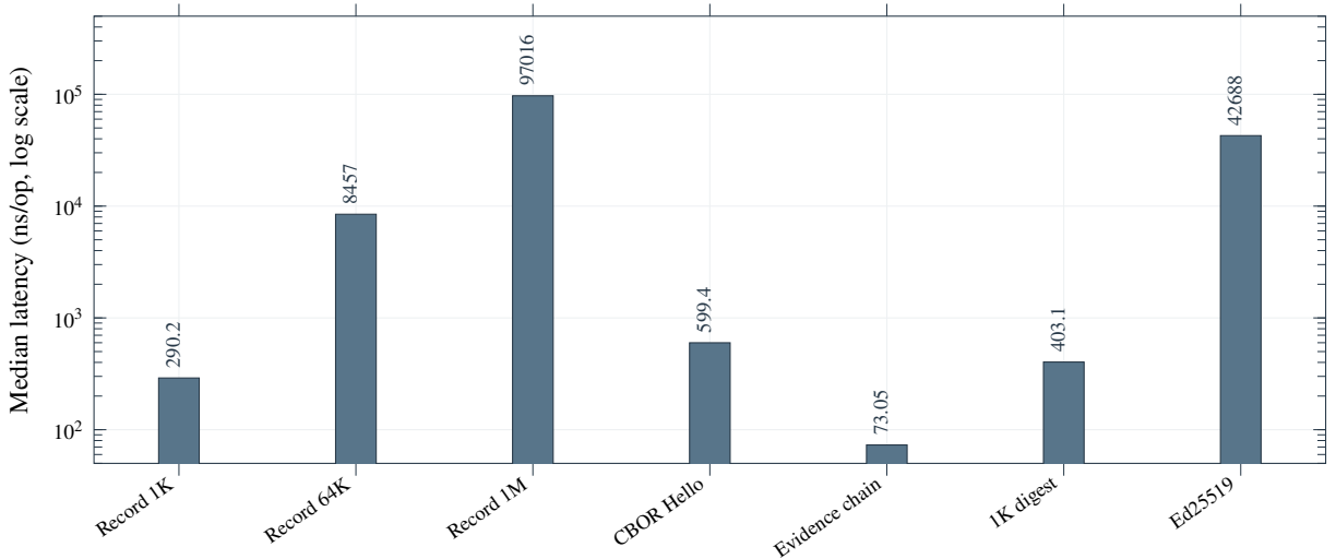
Figure 4: Empirical median latency of the seven measured in-memory primitives, read directly from the checked-in TSV and shown on a logarithmic axis. The isolated view makes the protocol’s CPU-side cost directly comparable with the interactive latency budget in Equation 7.
