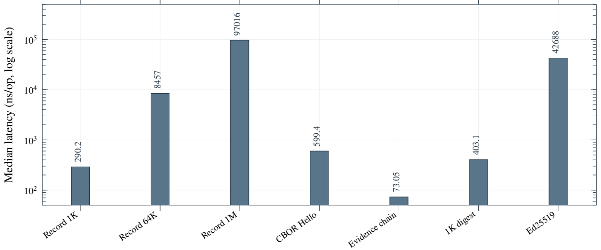
Figure 4: Empirical median latency of the seven measured in-memory primitives, read directly from the checked-in TSV and shown on a logarithmic axis; network, policy, storage, model, GPU, and token-generation costs are excluded. The isolated view makes the protocol’s CPU-side cost directly comparable with the interactive latency budget in Equation 7.
