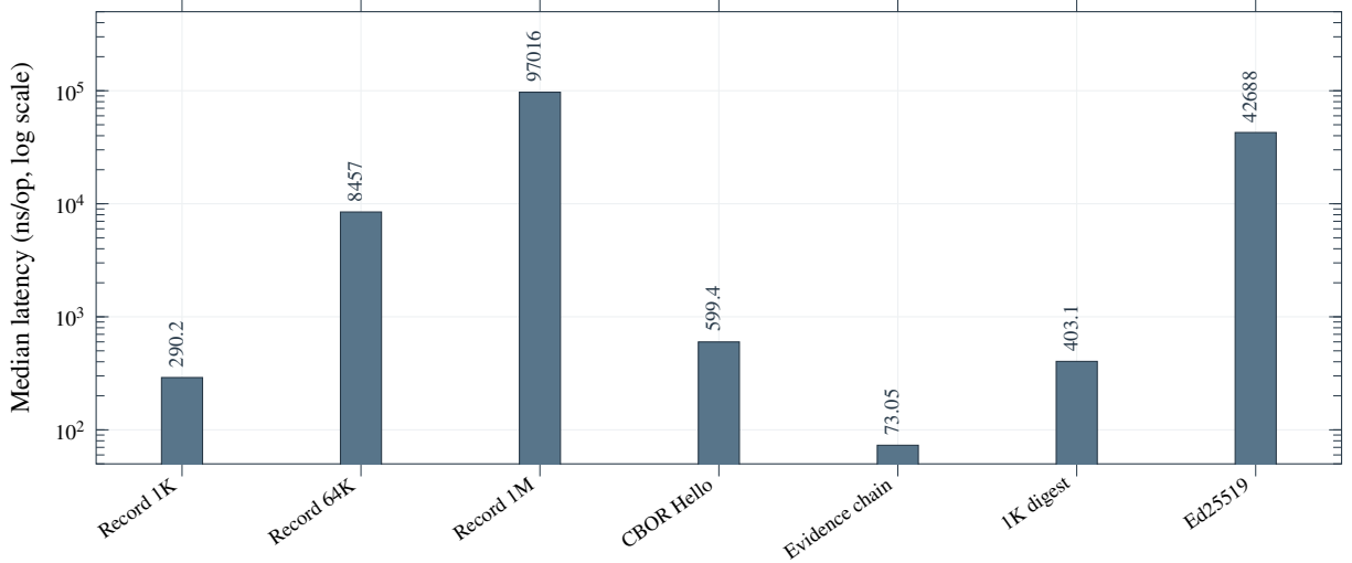
Figure 4: Empirical median latency of the seven measured in-memory primitives, read directly from the checked-in TSV and shown on a logarithmic axis. The plot excludes network, Relay policy, persistence, model, GPU, TTFT, and token-generation costs.
