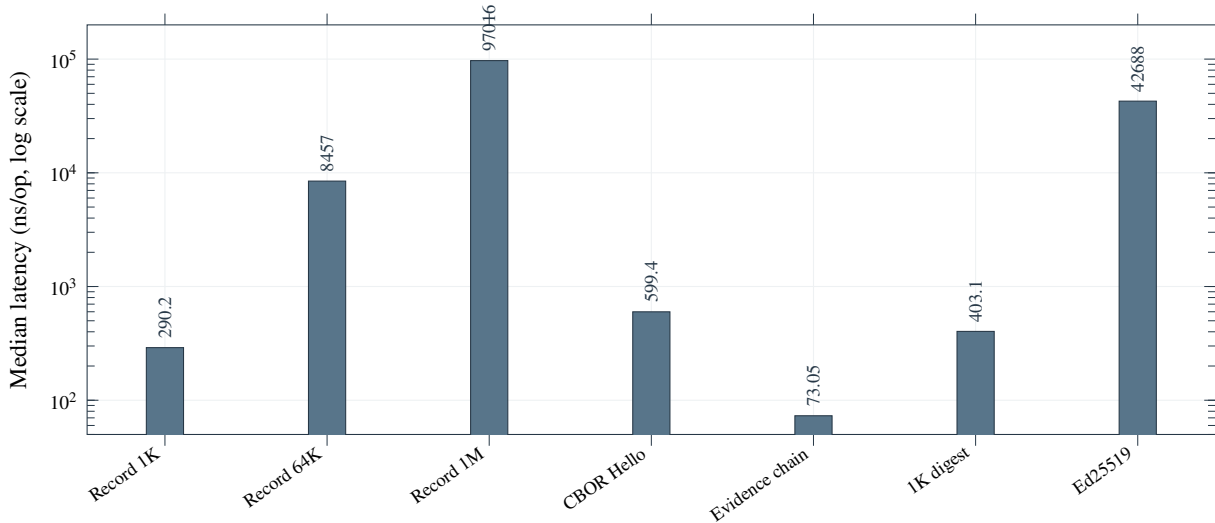
Figure 4: Empirical median latency of the seven measured in-memory primitives, read directly from the checked-in TSV and shown on a logarithmic axis. The plot excludes network, Relay policy, persistence, model, GPU, TTFT, and token-generation costs.
