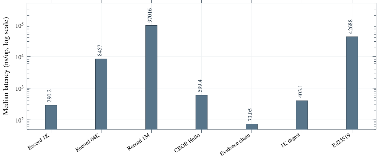
Figure 4: Empirical median latency of the seven measured in-memory primitives, read directly from the checked-in TSV and shown on a logarithmic axis. The isolated view makes the protocol’s CPU-side cost directly comparable with the interactive latency budget in Equation 6.
