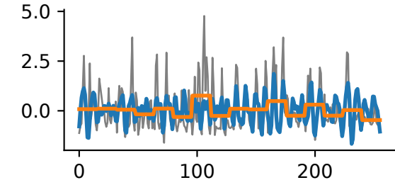
Iquique
