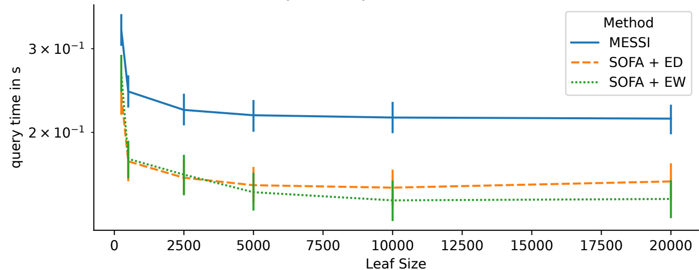
Mean Query times by Leaf Size (mixed workload)
