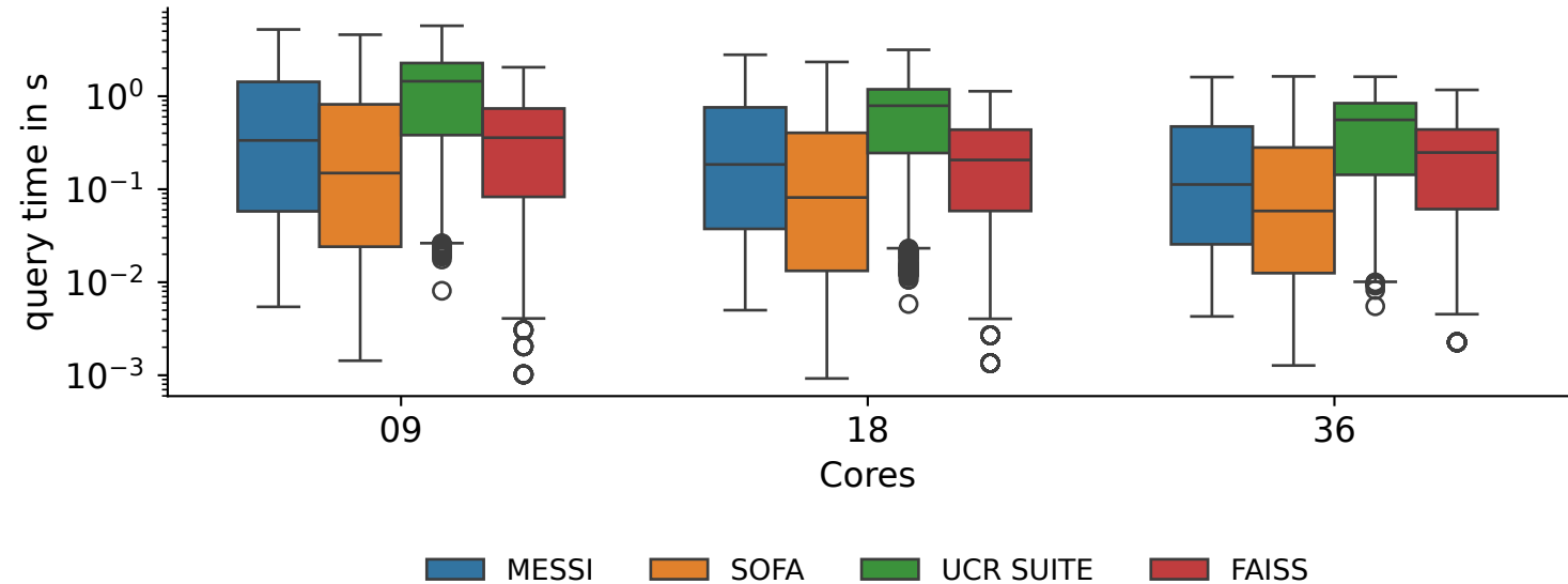
Mean Query times by #Cores (mixed workload)
