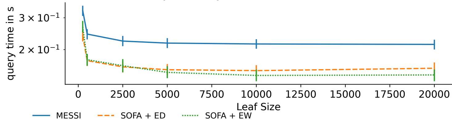
Query times by Leaf Size (mixed workload)
