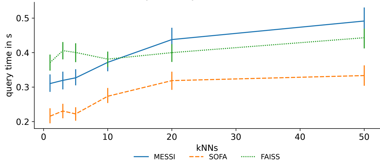
Mean Query times by #kNNs (mixed workload)
