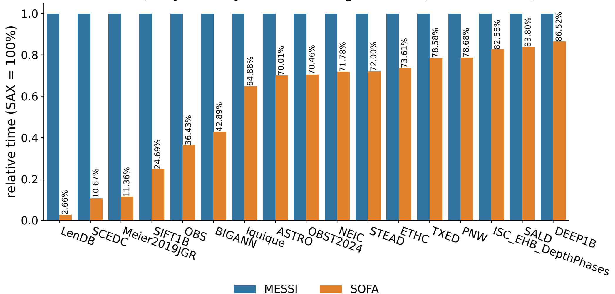
Relative Query Time by workload using 18 cores (lower is better)
