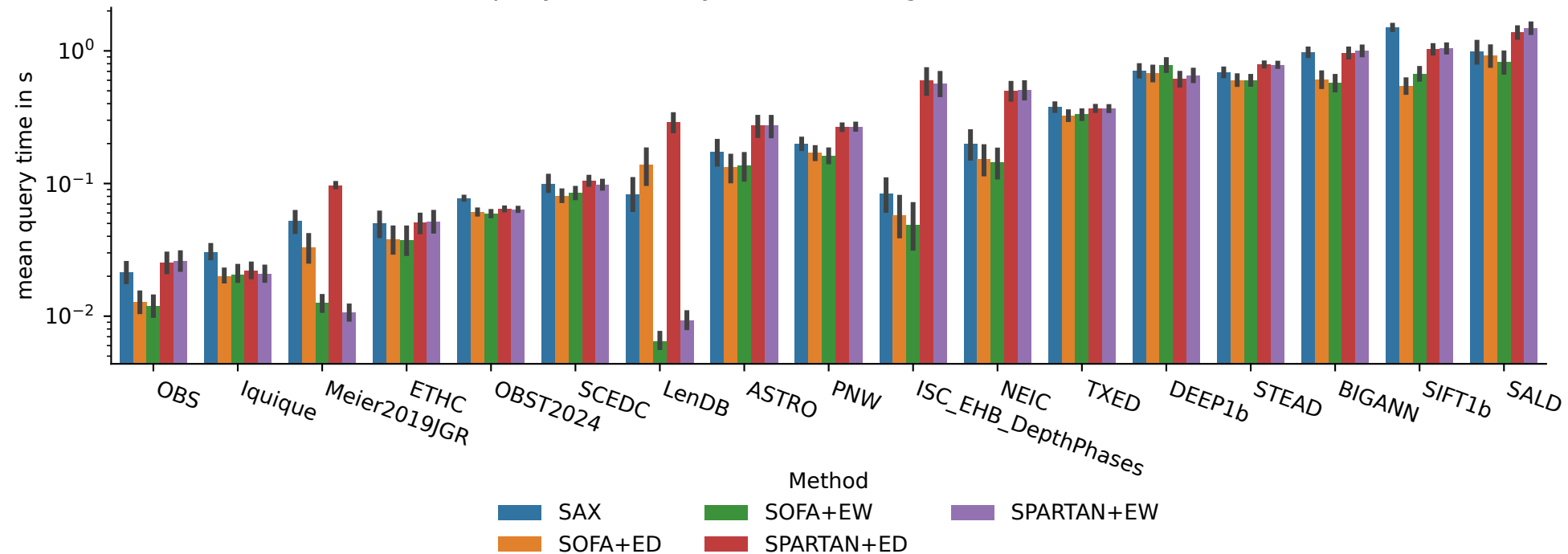
Mean query time in s by workload using 36 cores (lower is better)
