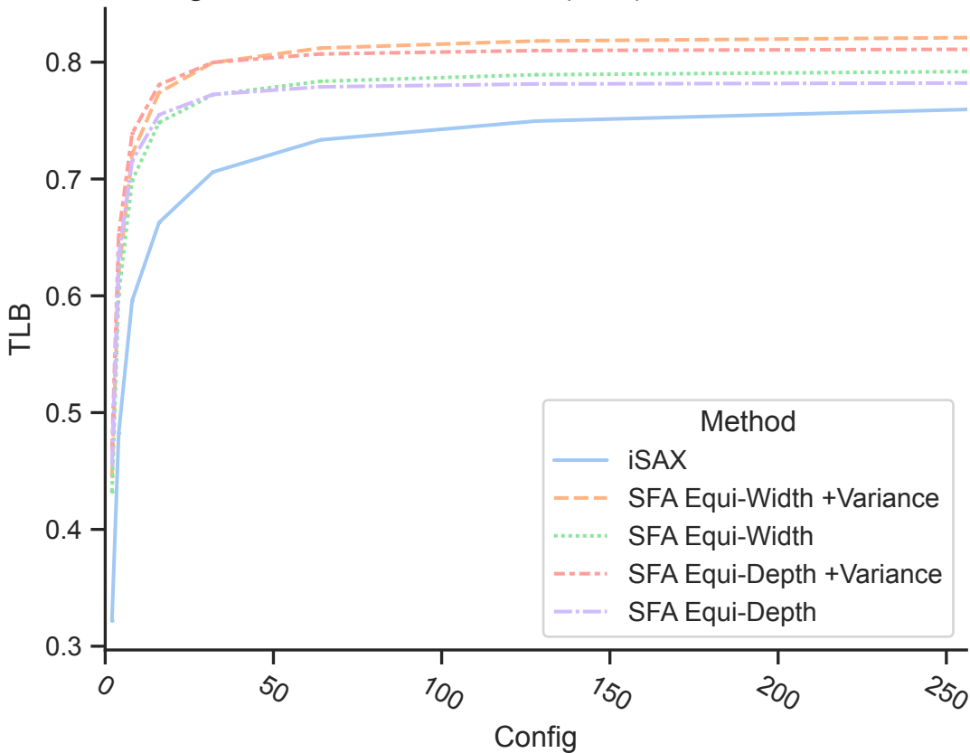
Tightness of Lower Bound (TLB) on UCR datasets
