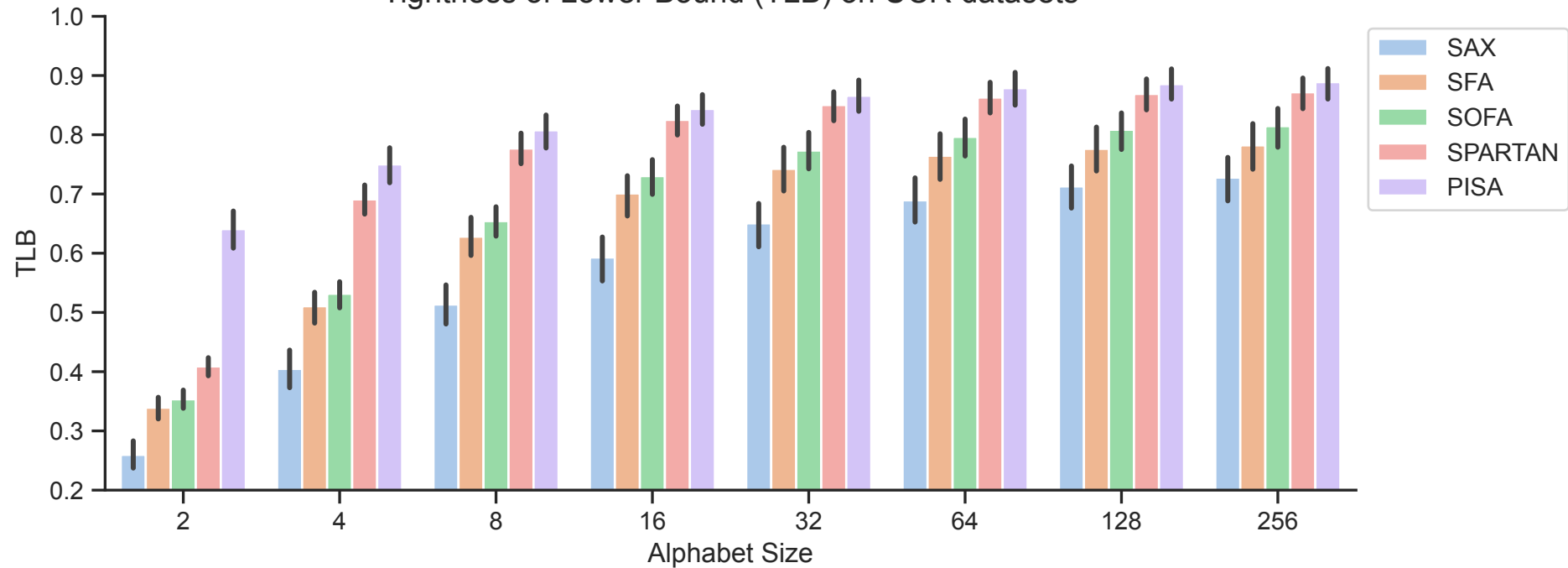
Tightness of Lower Bound (TLB) on UCR datasets
