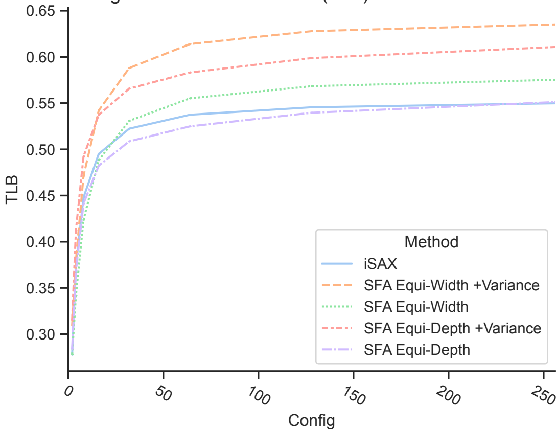
Tightness of Lower Bound (TLB) on SOFA datasets
