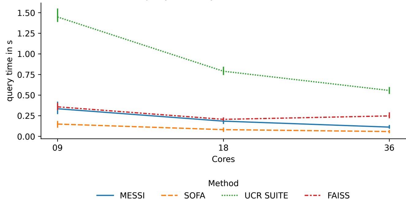
Median query times by #Cores (mixed workload)
