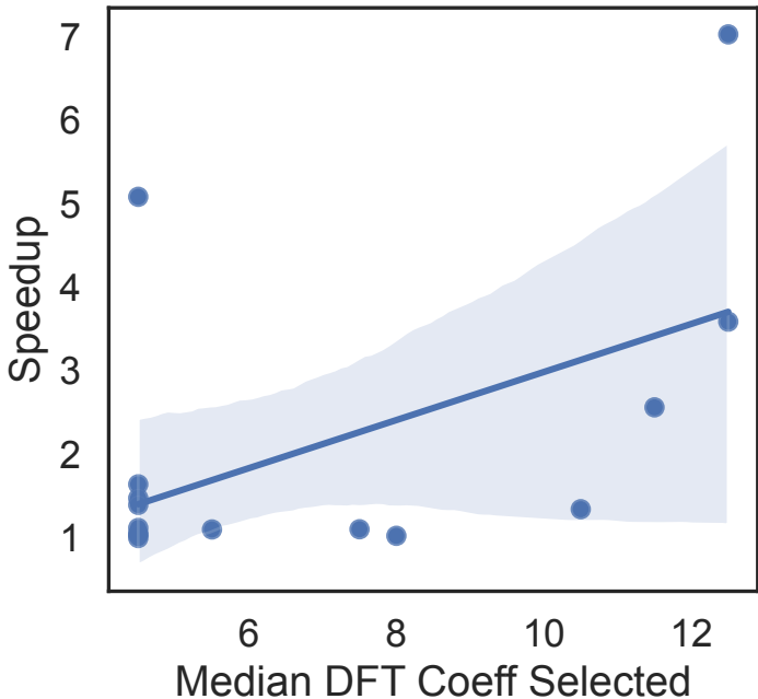
Speedup SOFA over MESSI
