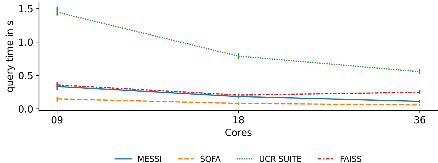
Median Query times by #Cores (mixed workload)
