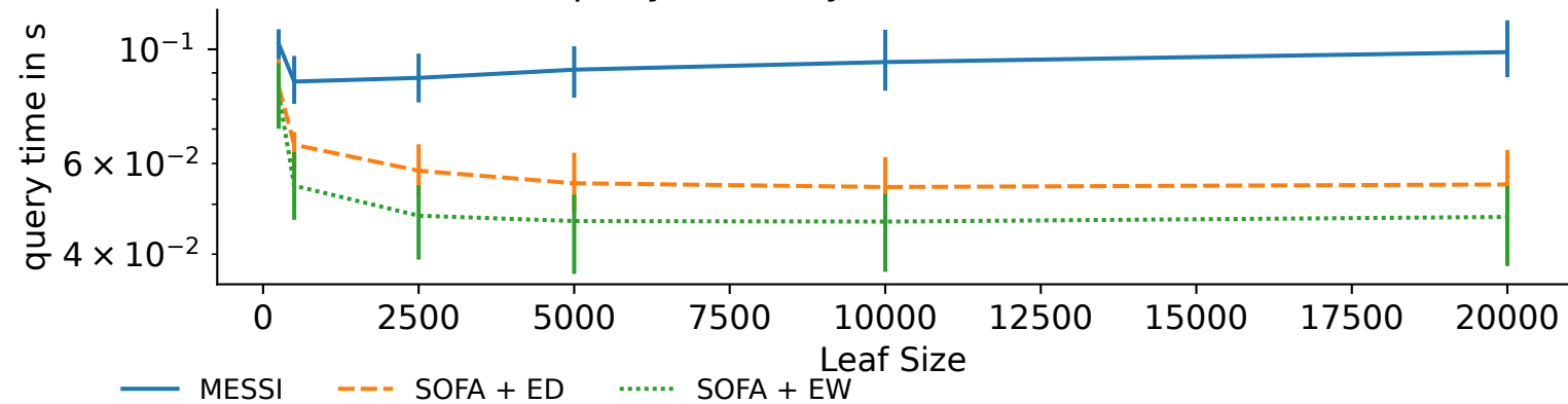
Median query times by Leaf Size (mixed workload)
