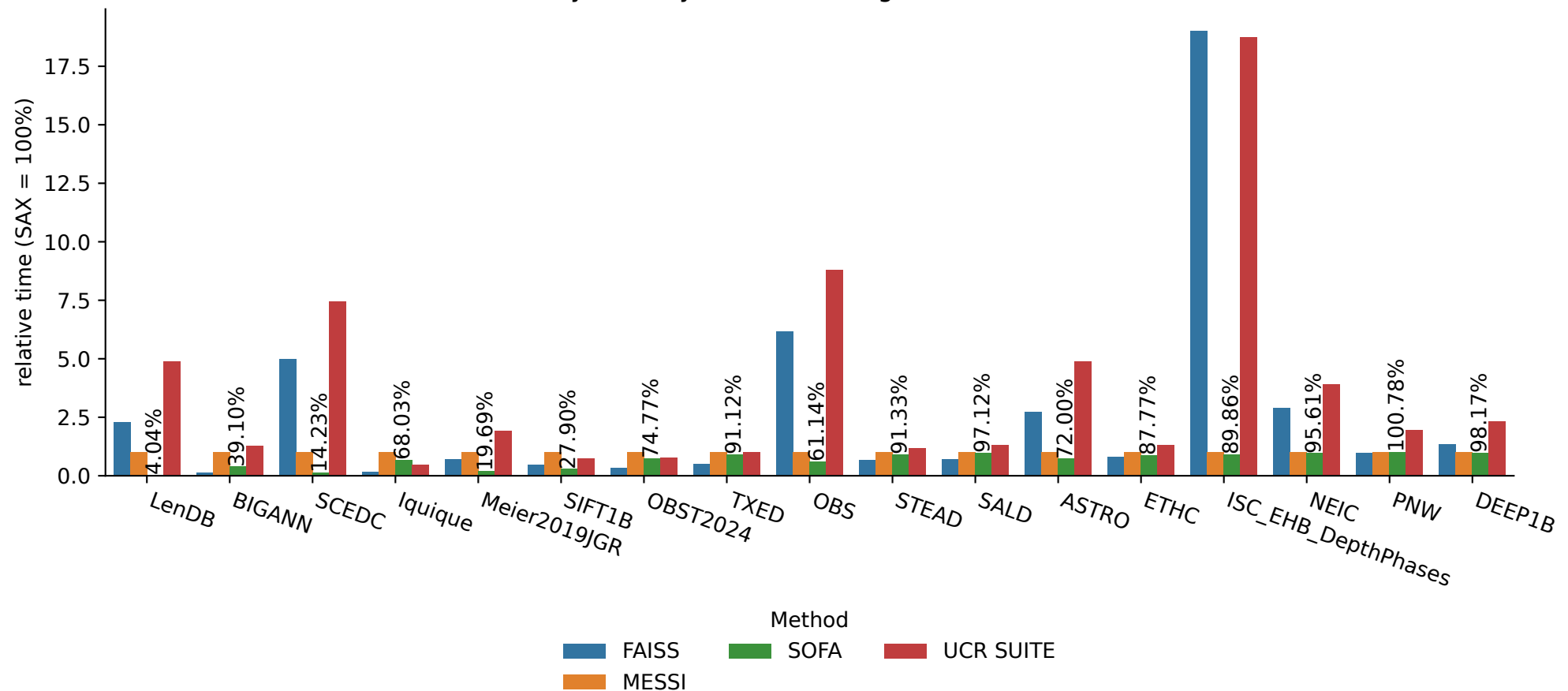
Relative Query Time by workload using 36 cores (lower is better)
