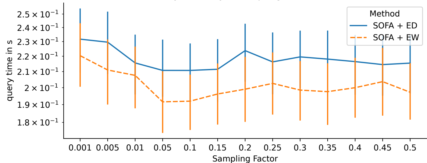
Mean Query times by #Sampling (mixed workload)
