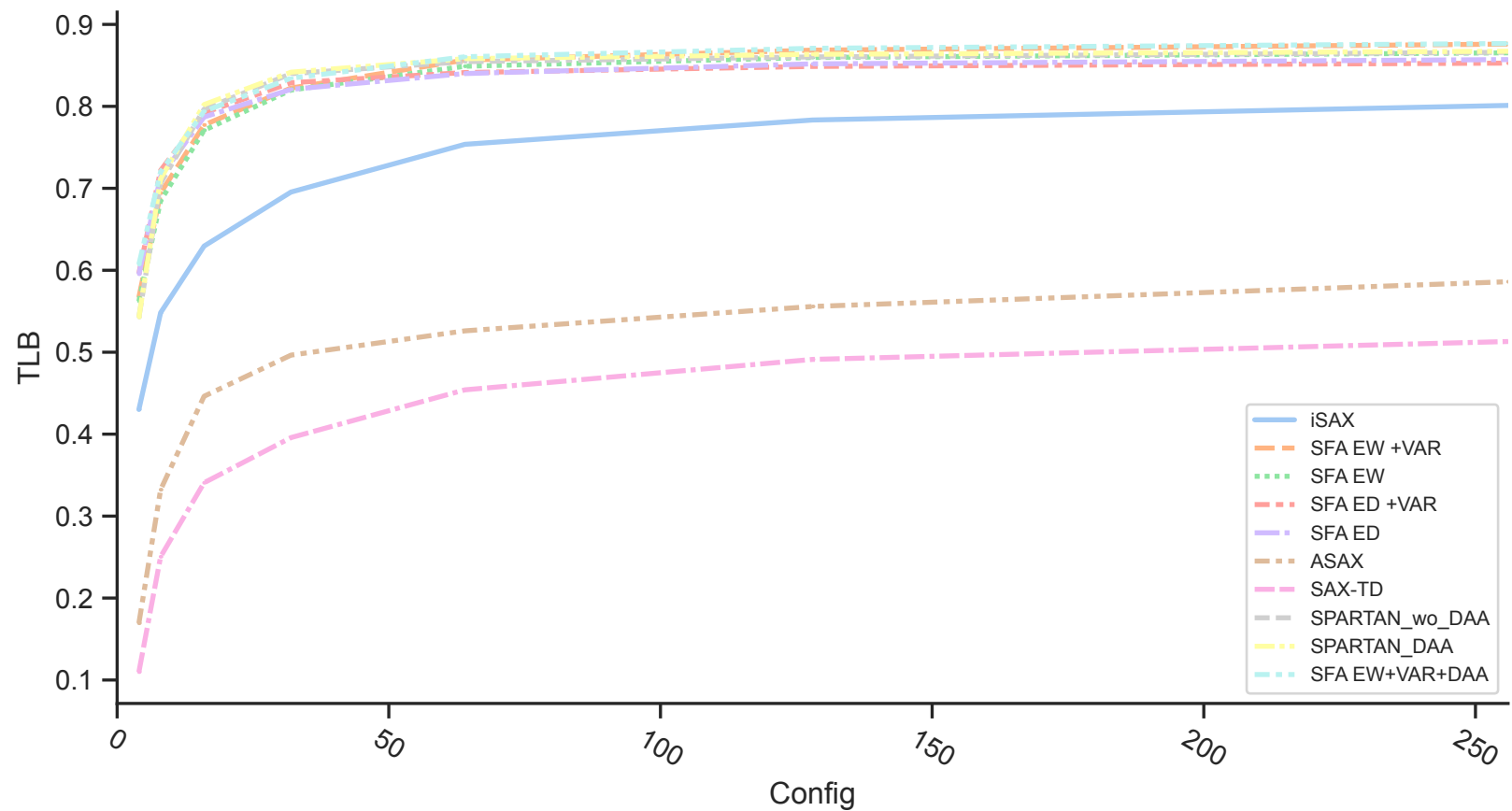
TLB on UCR datasets
