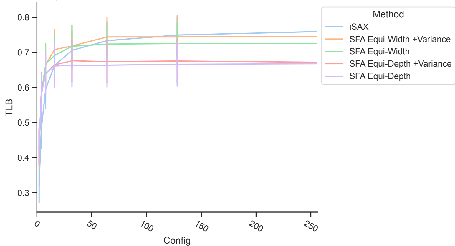
Tightness of Lower Bound (TLB) on 118 UCR datasets
