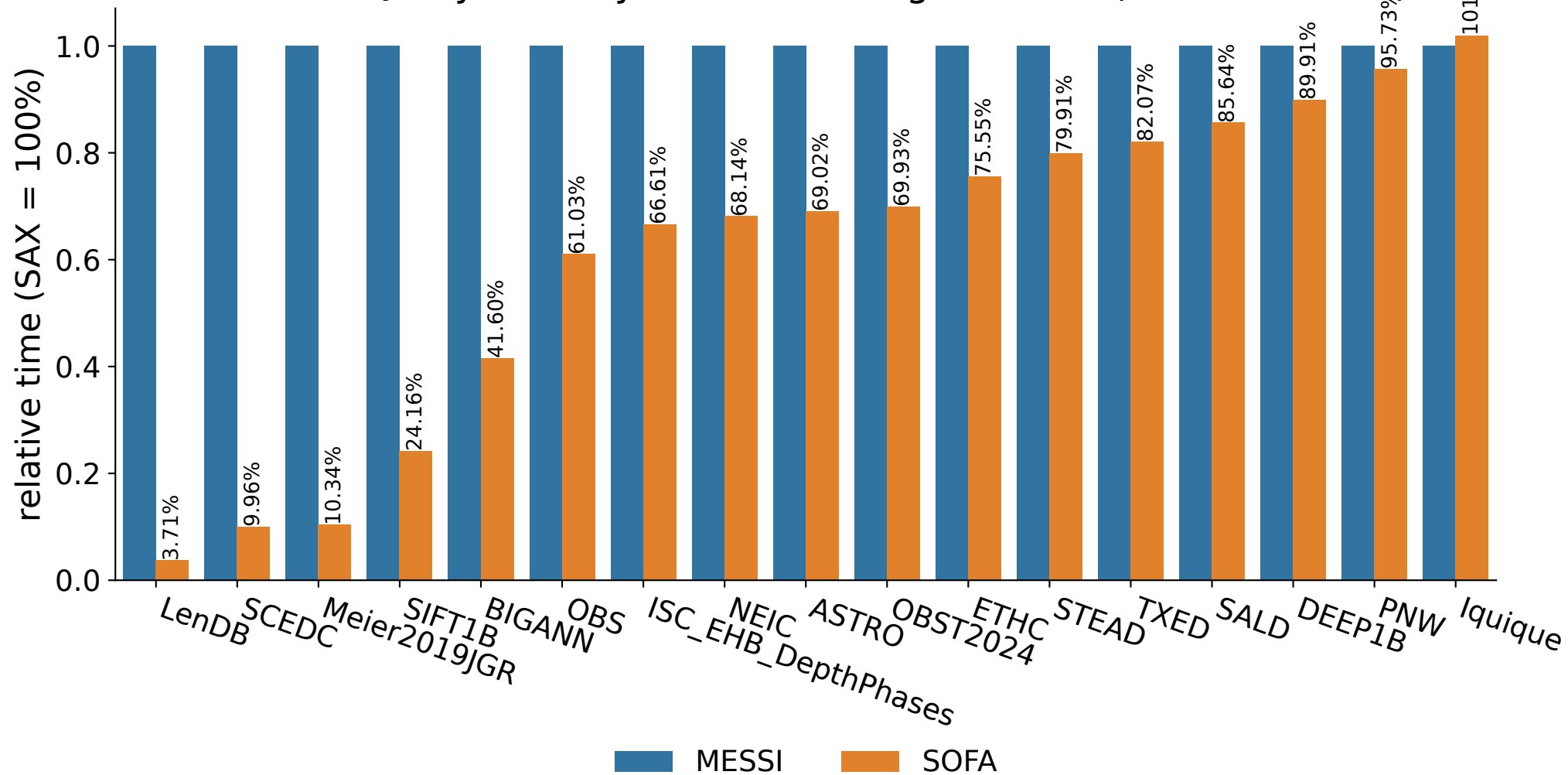
Relative Query Time by workload using 09 cores (lower is better)
