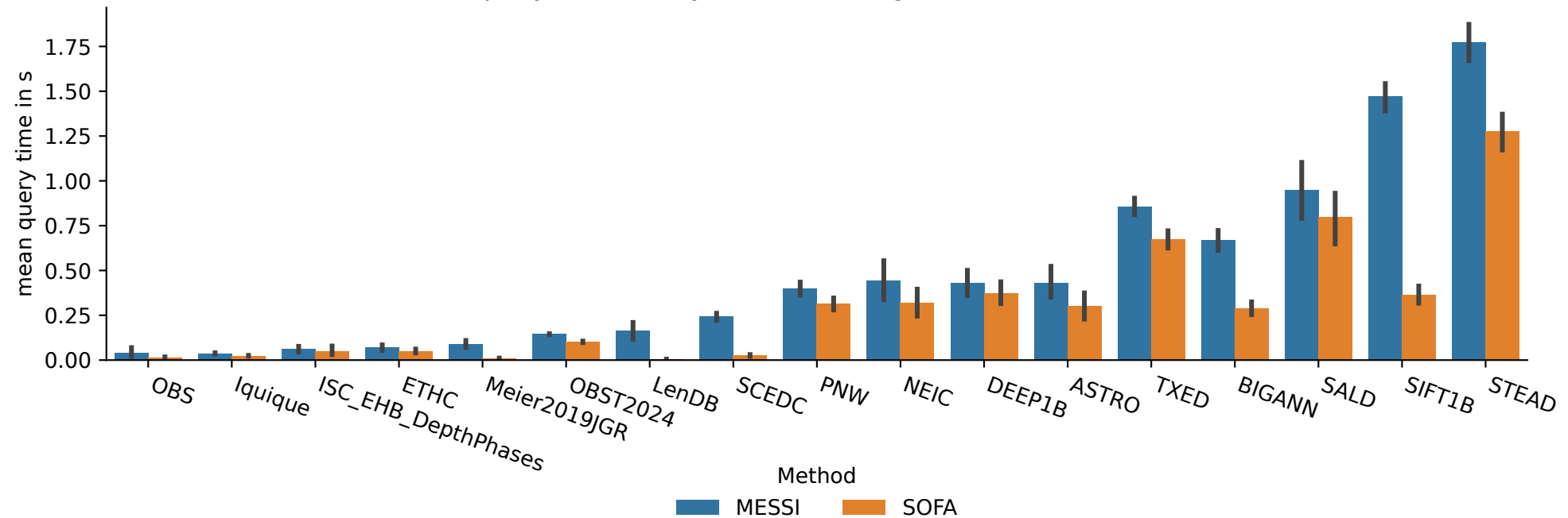
Mean query time in s by workload using 18 cores (lower is better)
