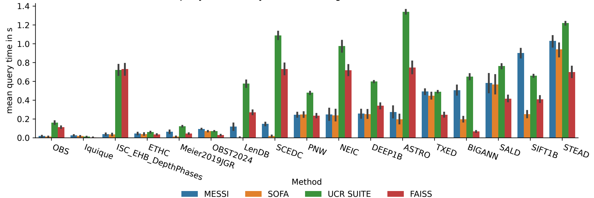
Mean query time in s by workload using 36 cores (lower is better)
