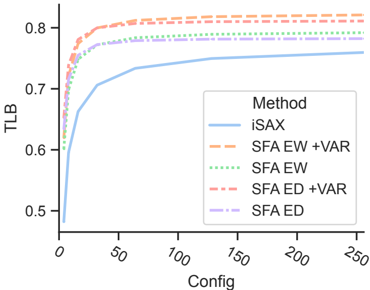
TLB on UCR datasets
