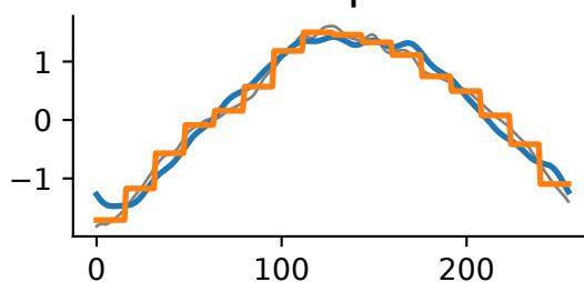
deep1b
