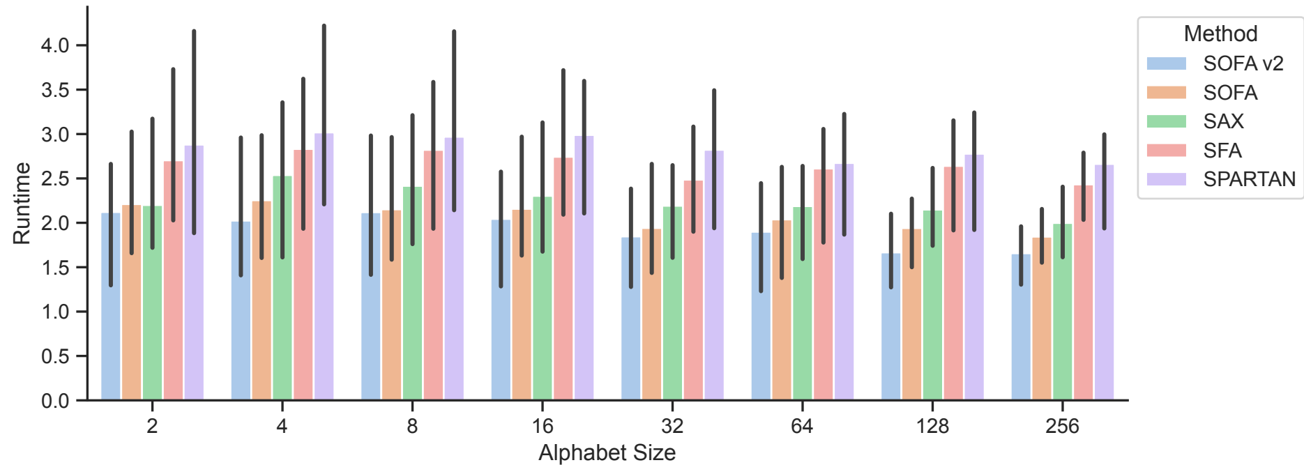
Median Runtime on UCR datasets
