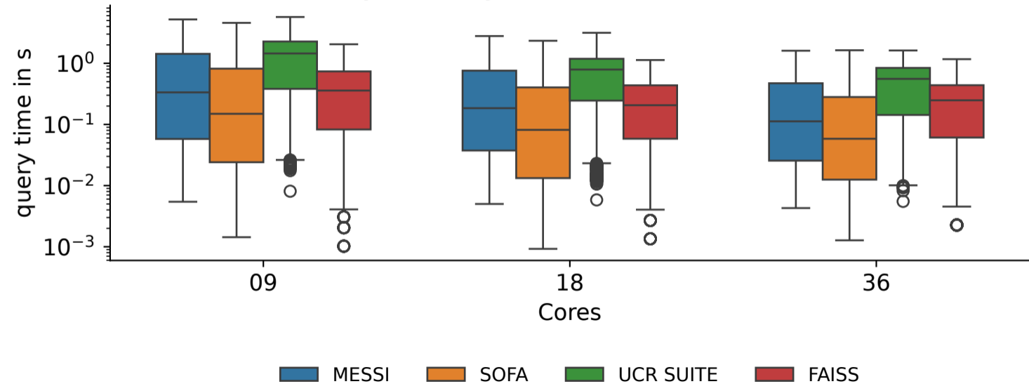
Query times by #Cores (mixed workload)
