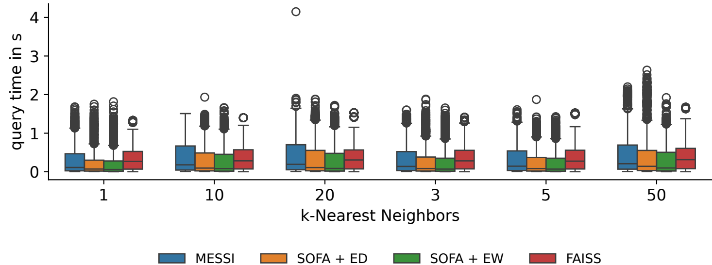
Query times by #kNNs (mixed workload)
