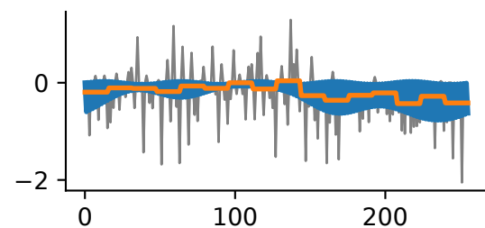
NEIC
