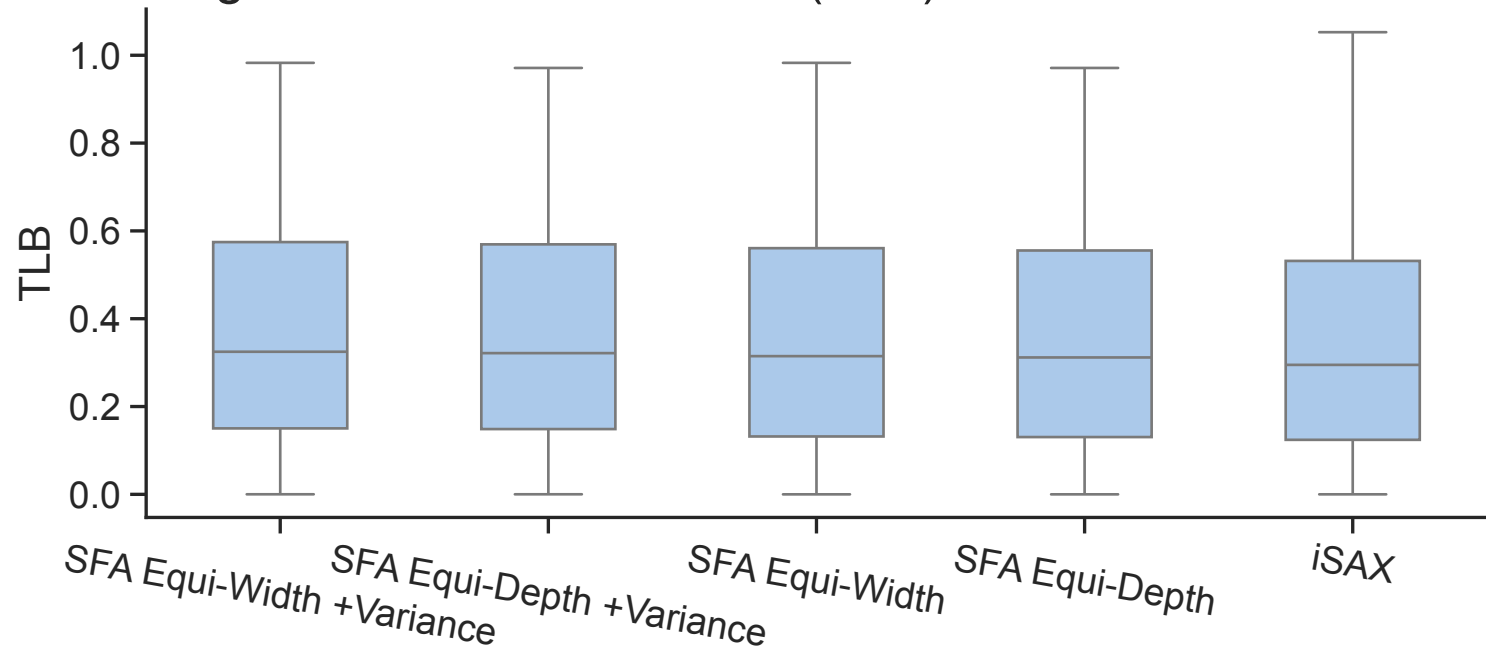
Tightness of Lower Bound (TLB) on 118 UCR datasets
