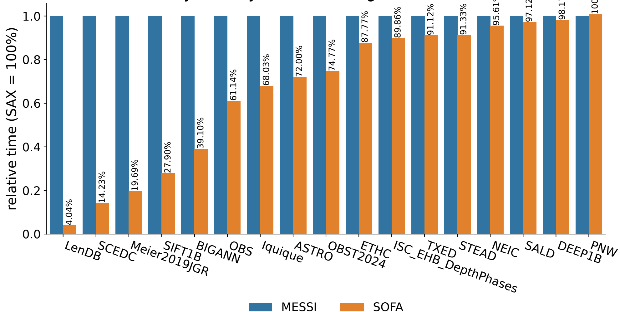
Relative Query Time by workload using 36 cores (lower is better)
