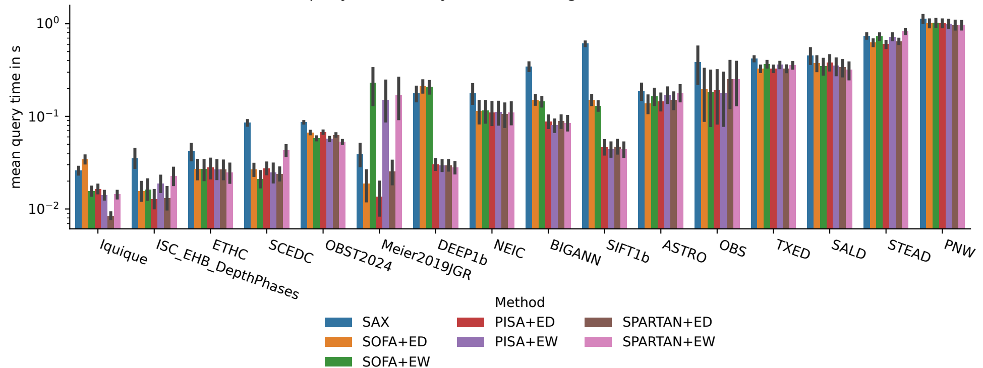
Mean query time in s by workload using 36 cores (lower is better)
