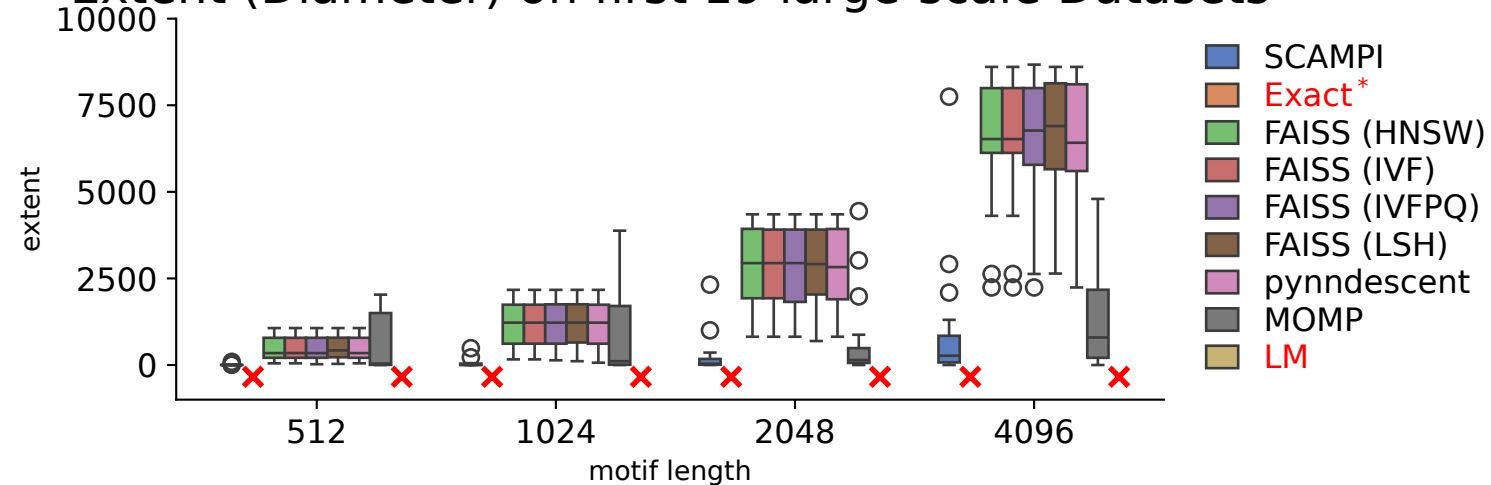
Extent (Diameter) on first 19 large-scale Datasets
