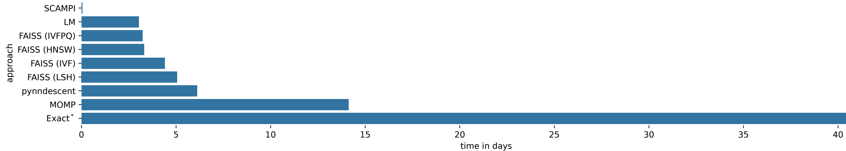
Total Runtime in Days along 19 Datasets
