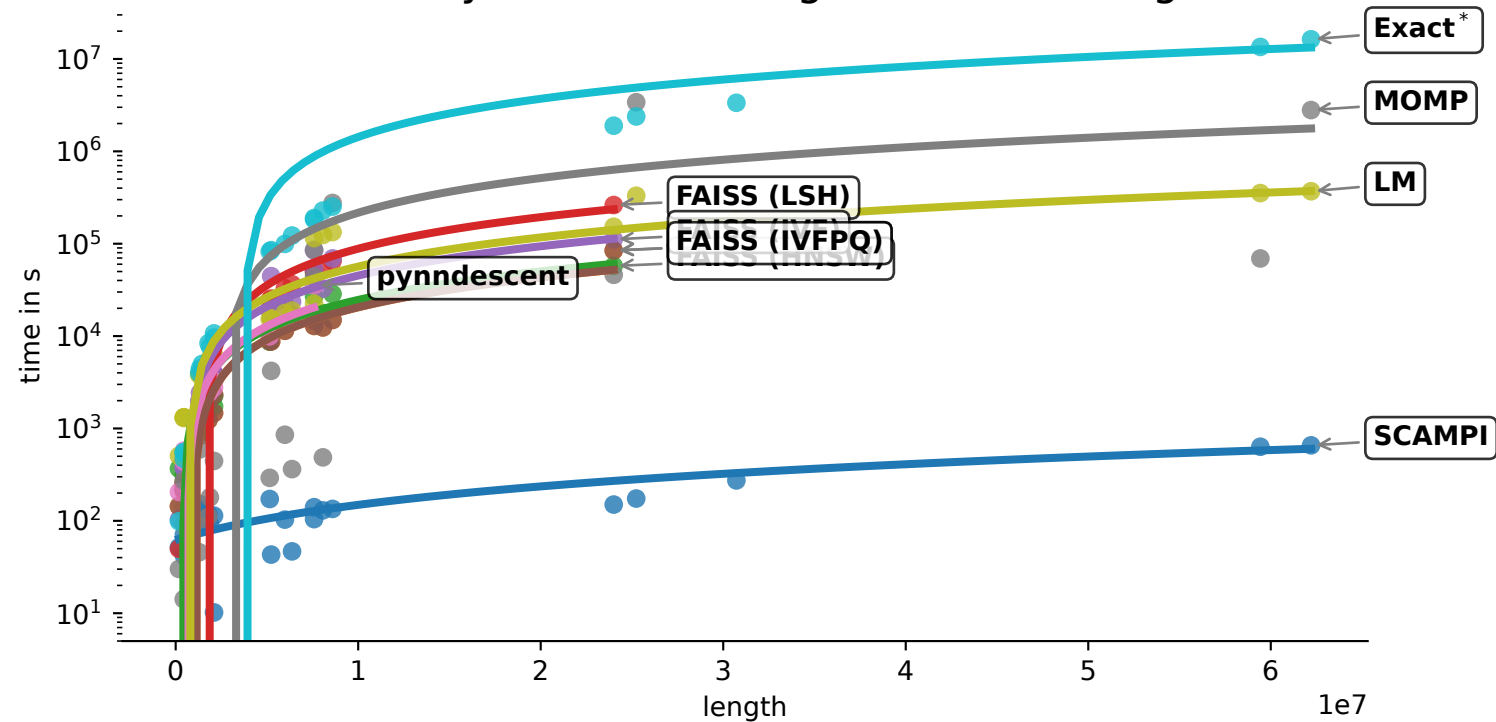
Scalability with increasing time series length
