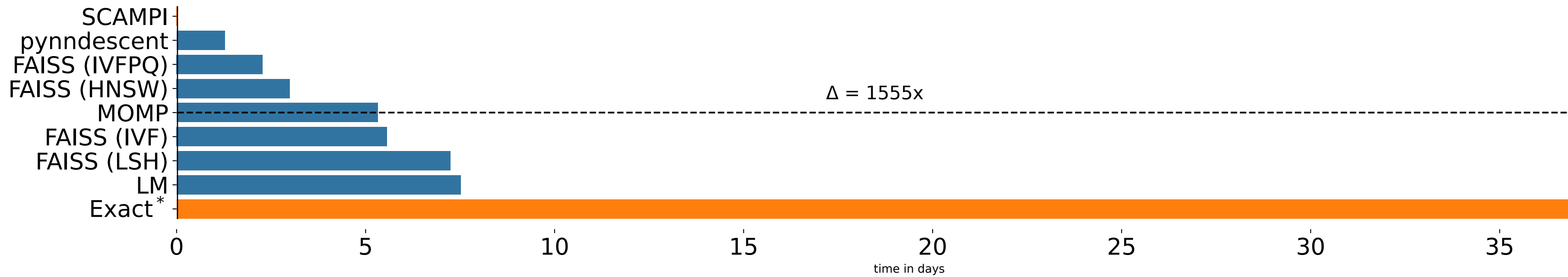
Total Runtime in Days - over 20 Datasets
