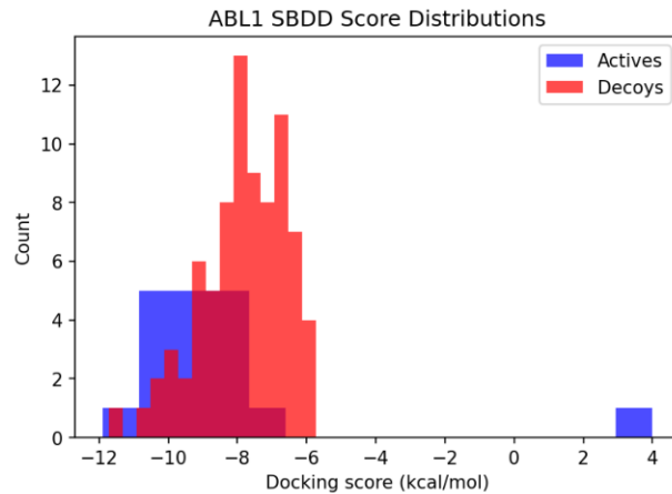
ABL1 Docking Score Distributions
