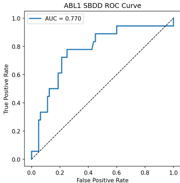
ABL1 SBDD ROC Curve
