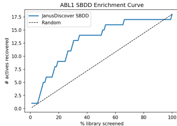
ABL1 SBDD Enrichment Curve
