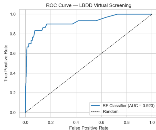
(b) ROCK2 (MUV-644) — ROC curve
