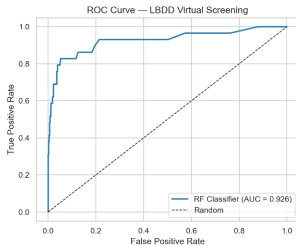
(a) PKA (MUV-548) — ROC curve
