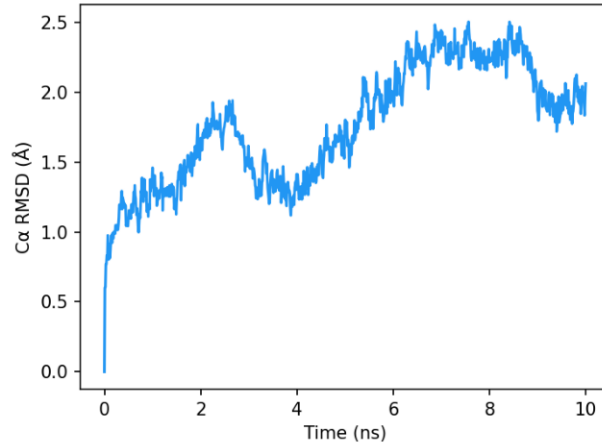
(a) Ca RMSD vs Time
