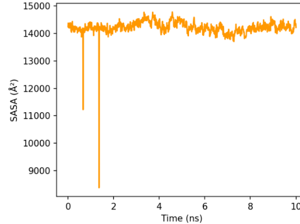
(e) SASA vs Time
