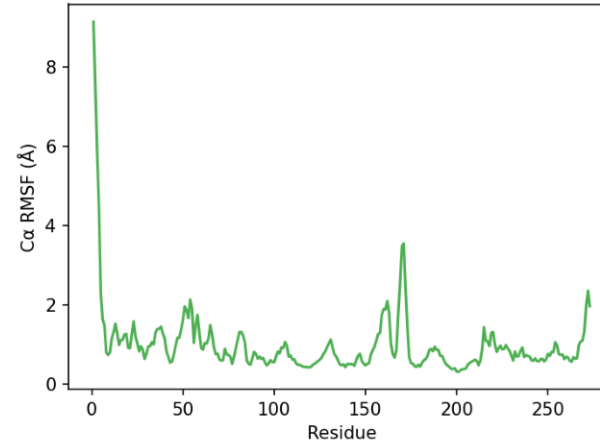
(b) Per-residue RMSF
