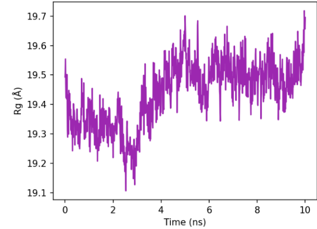
(c) Radius of Gyration
