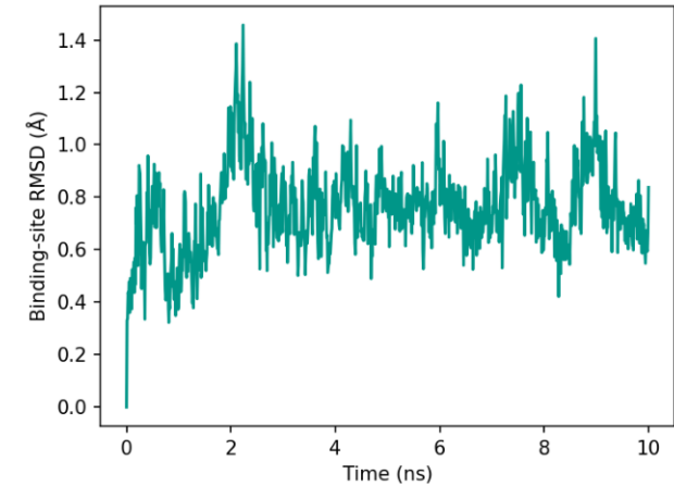
(f) Binding-site RMSD
