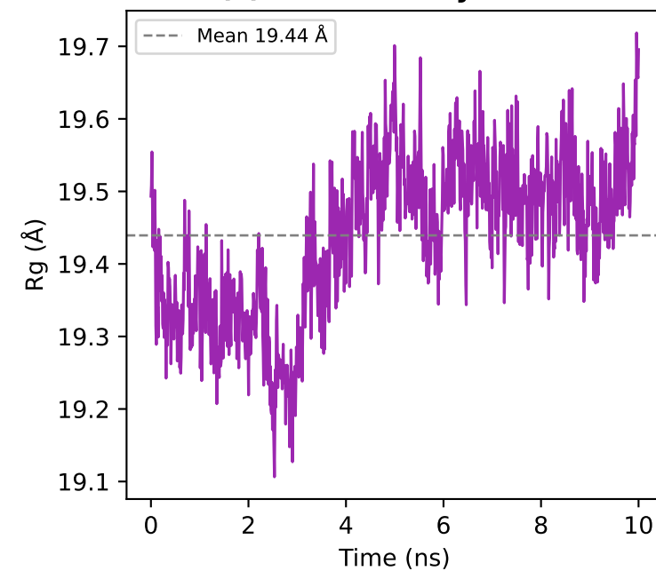
(c) Radius of Gyration
