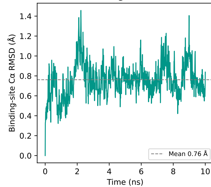
(f) Binding-site RMSD
