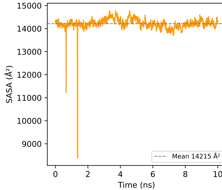
(e) SASA vs Time
