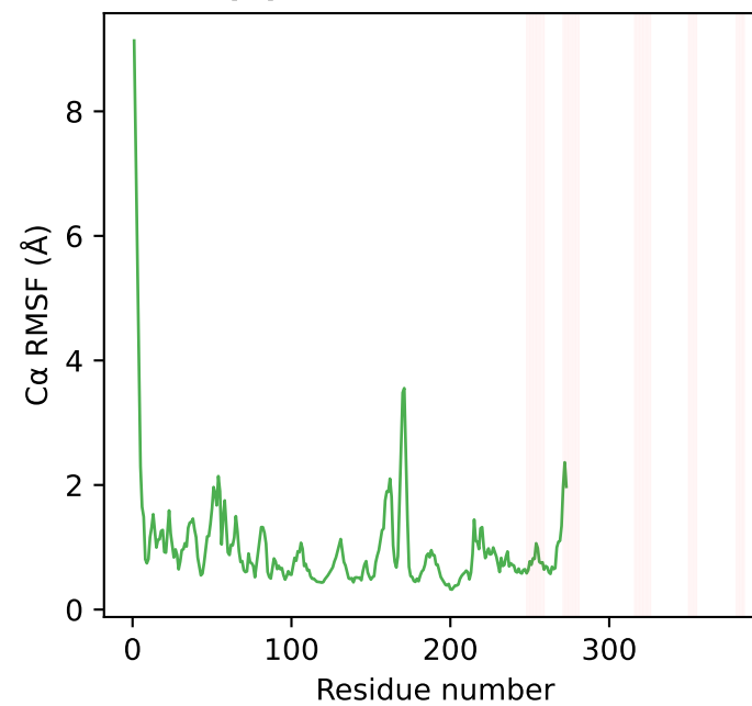
(b) Per-residue RMSF
