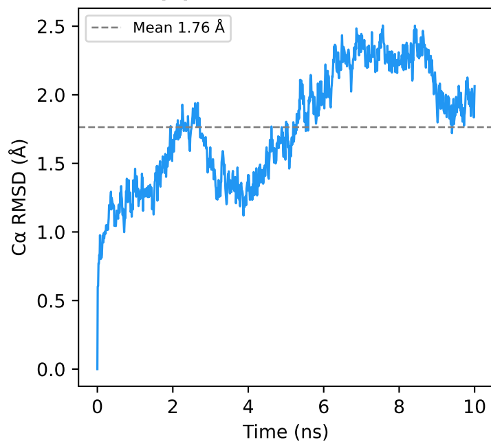
(a) C \alpha RMSD vs Time
