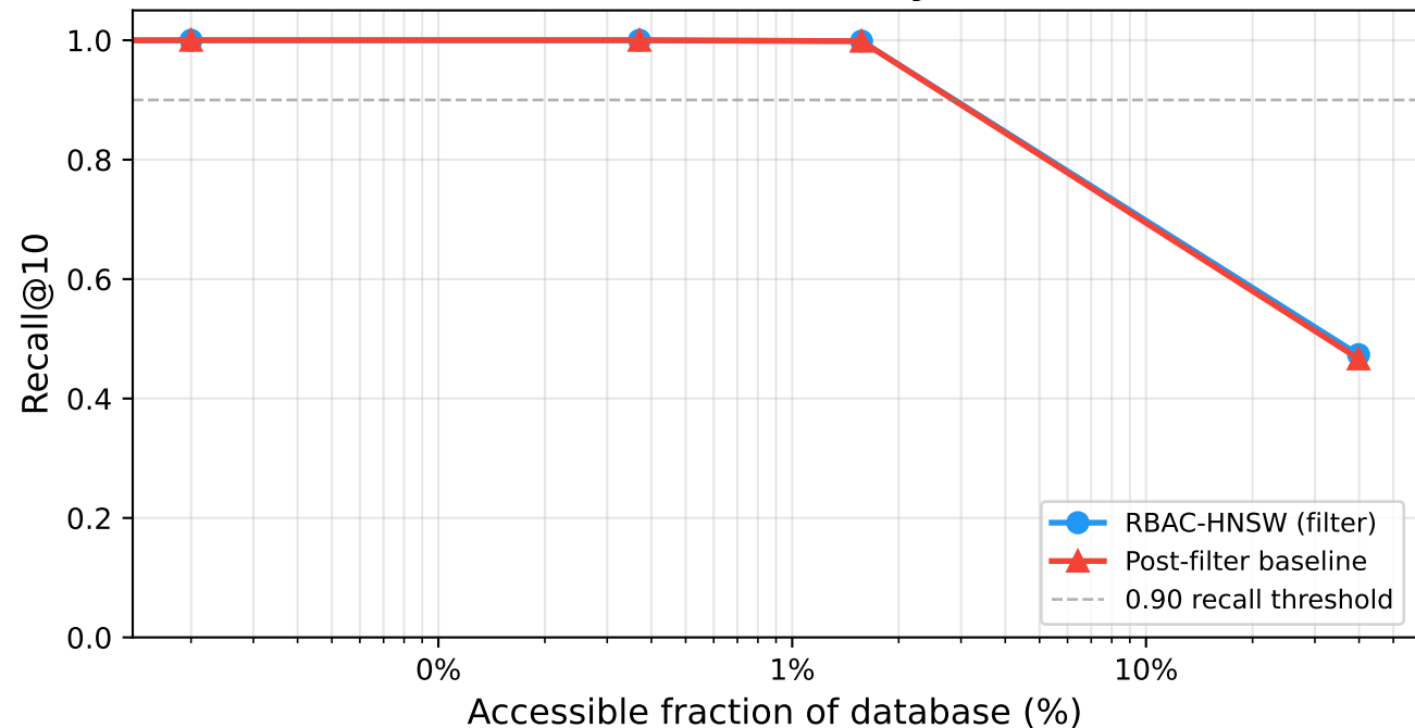
Recall@10 vs. Selectivity (ef=200)
