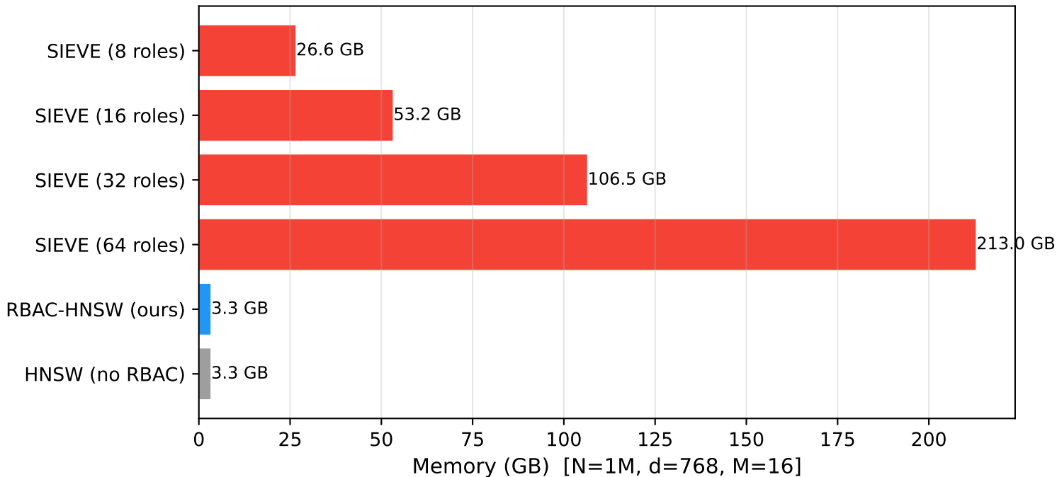
Memory Footprint Comparison (1M vectors)
