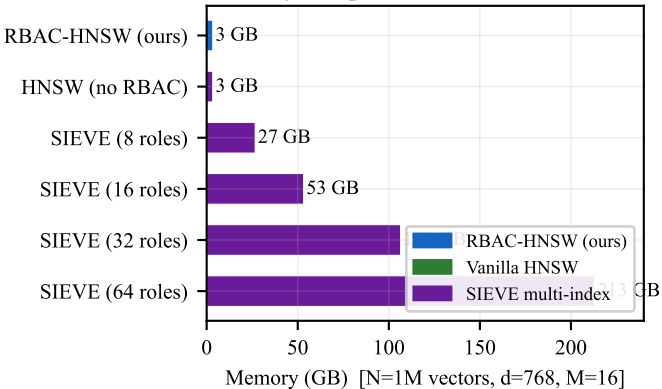
Memory Footprint vs. SIEVE Multi-Index
