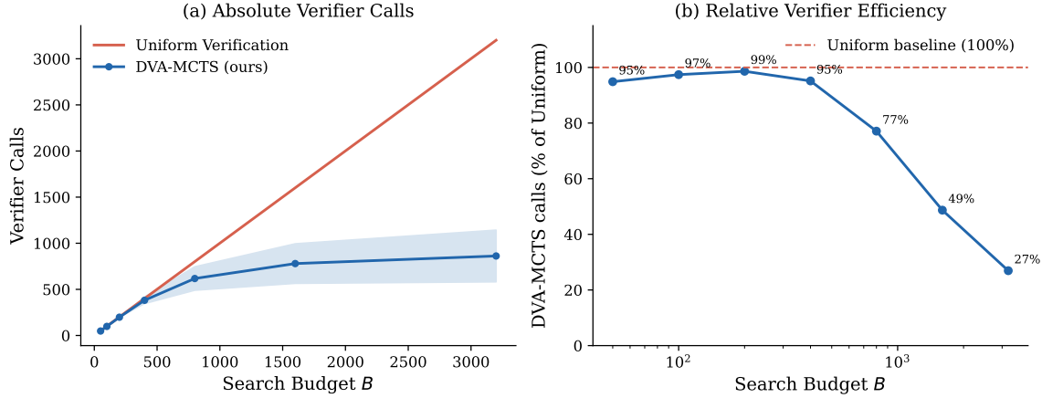
Figure 2: Verifier call efficiency as a function of search budget B (range B=50 – 3,200 ; all data in the transition regime, B < N_{\mathcal{T}}=8,190 ). (a) Absolute verifier calls: DVA-MCTS is bounded by the theoretical ceiling N_{\mathcal{T}} = K(K^D - 1)/(K - 1) (constant, independent of B ). In the transition regime, empirical counts grow as \approx 1.9\sqrt{B} \log B as the Lipschitz proxy substitutes for increasingly many first-visit calls. (b) DVA-MCTS calls as a fraction of Uniform, showing increasing efficiency from \approx 5\% savings at B=400 to 73\% at B=3,200 . Full exploitation-regime savings ( 93.7\% at B=16,384 ) are shown in Table 1 (Section 6.5).
