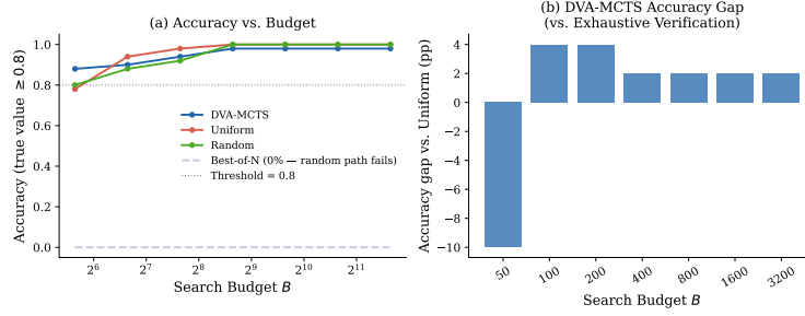
Figure 4: Compute-accuracy tradeoff (50 runs per budget; transition regime, B=50\text{--}3,200 < N_T=8,190 ). DVA-MCTS matches Uniform Verification within 2 percentage points at all B \geq 400 while using up to 73% fewer verifier calls at B=3,200 (proxy mechanism). Random-path Best-of- N fails in deep trees (0% accuracy; see Section 6.8).
