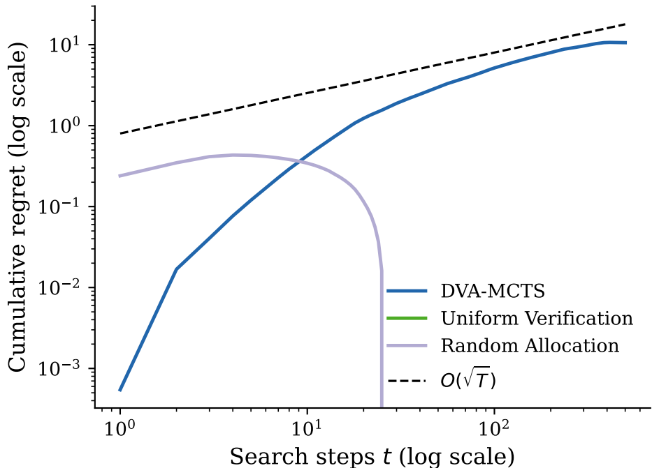
(b) Log-Log Scaling
