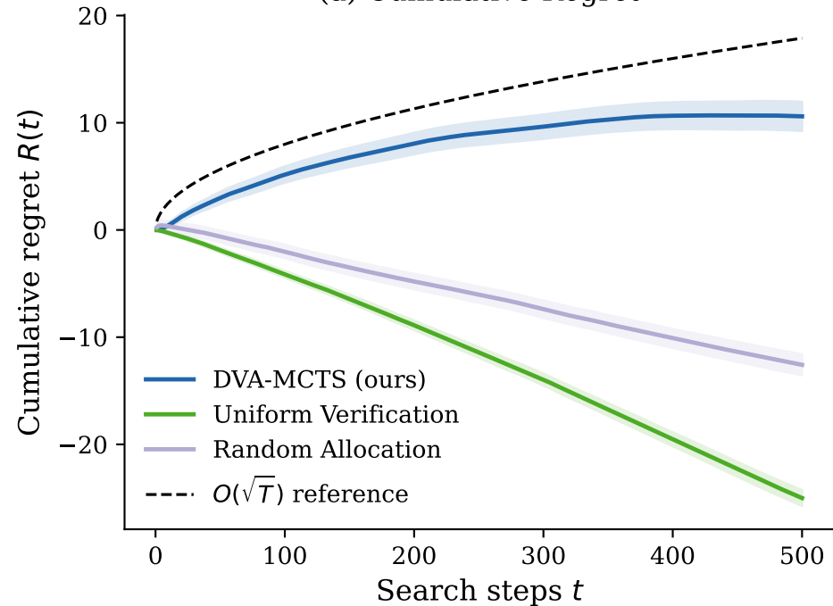
(a) Cumulative Regret
