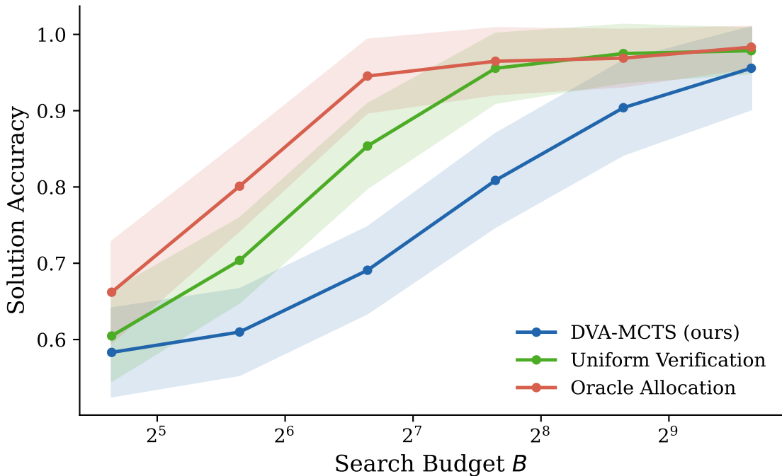
Compute-Accuracy Tradeoff
