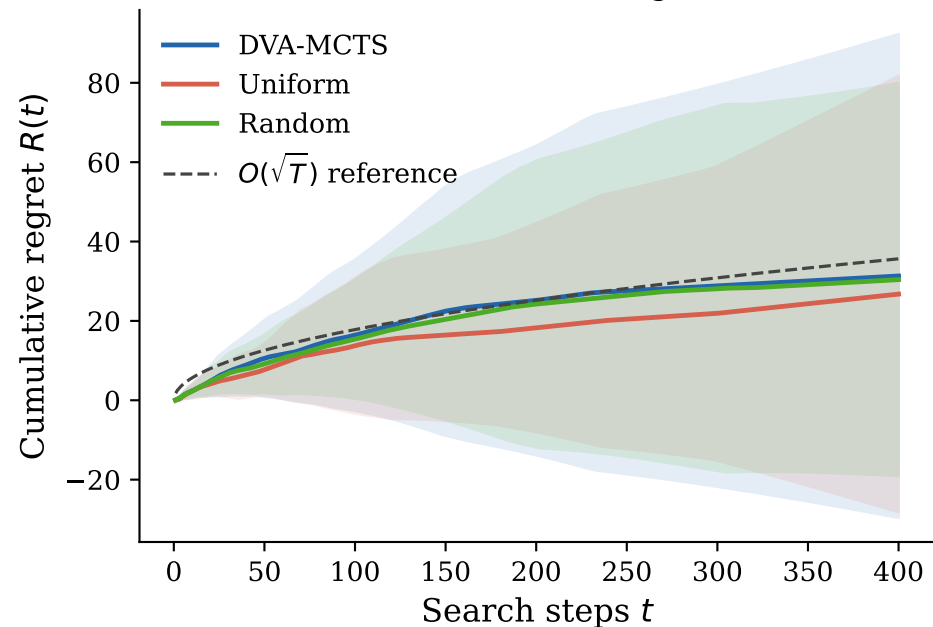
(a) Cumulative Regret
