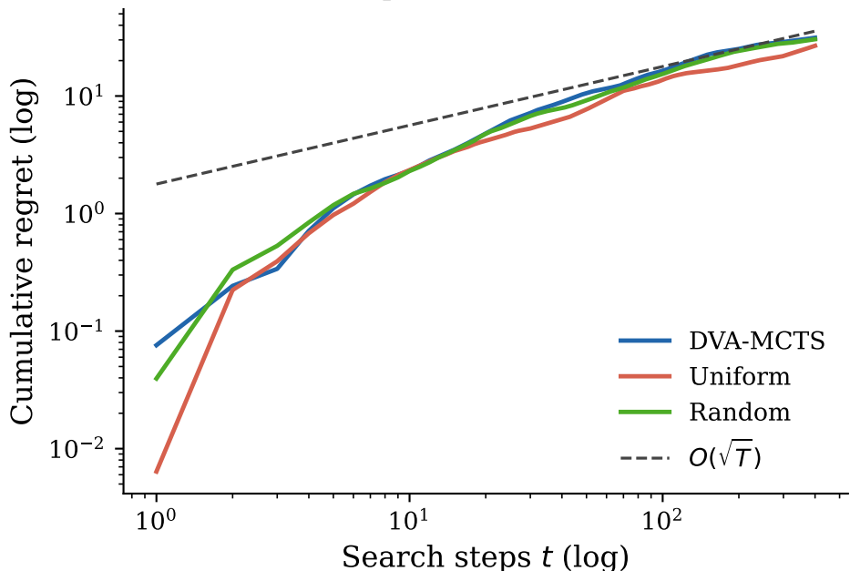
(b) Log-Log Scaling DVA-MCTS exponent = 0.635 ( R^2 = 0.961 )
