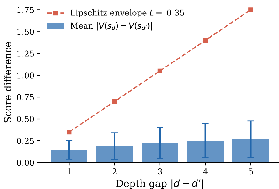
(a) Score Differences vs. Depth Gap Envelope never violated (0 of 22,500 pairs)
