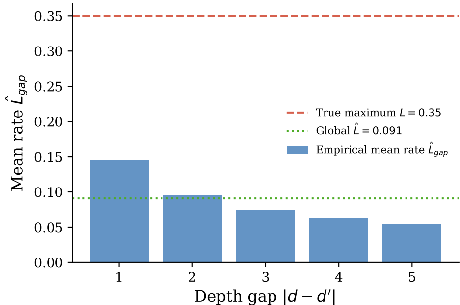
(b) Mean Rate vs. Lipschitz Constant \hat{L} estimates mean rate; L is the supremum
