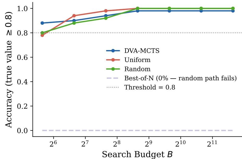
(a) Accuracy vs. Budget
