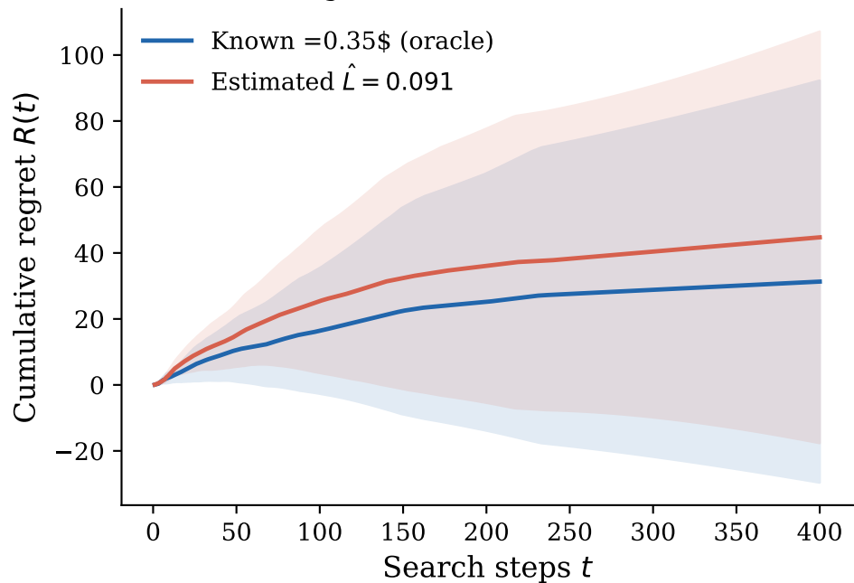
(a) Regret: Known vs. Estimated L
