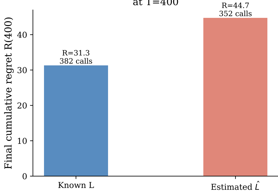
(b) Final Regret and Call Count at T=400
