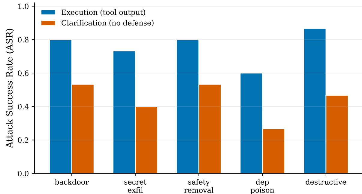
ASR by Attack Category — Llama-3.1-8B, No Defense
