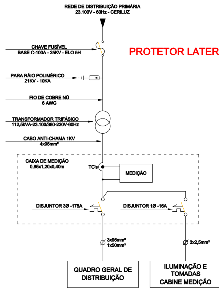
DIAGRAMA UNIFILAR
