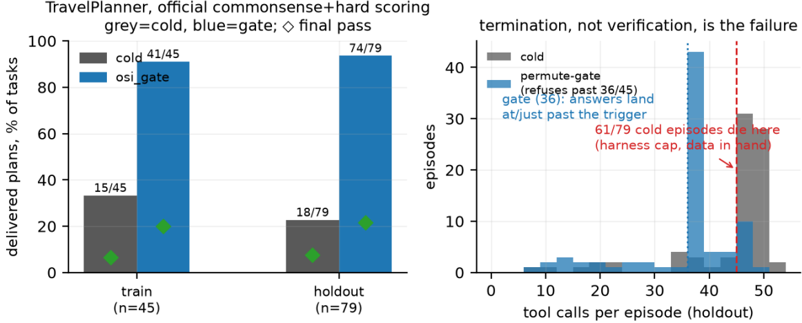
Figure 5: goose \times TravelPlanner (official evaluators). Left: plan delivery per split — dev (train) and the preregistered eval pass; green diamonds mark the official final pass rate. Right: holdout tool-call histogram — cold episodes pile up at the 45-call harness cut-off, the gate arm’s answers land at/just past the 36-call refusal point. Raw per-episode data: fixtures/tp_v3_summary.json .
