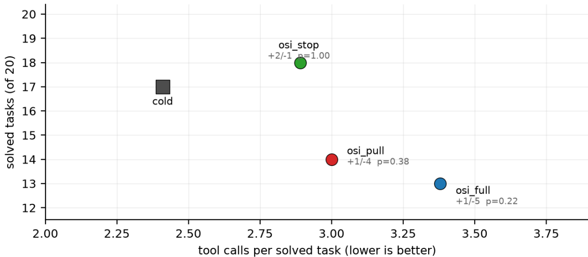
Figure 3: Cross-agent replication on goose: solved tasks vs. tool calls per solve, four arms, same tasks/scoring/model as the Hermes-side arms. Annotations give paired discordants against cold and exact McNemar p . The sentinel emitted no recurrence note on any episode (failures were one-off classes), yet pull-based access still cost solves — the tax is in the prompting, not in the notes.
