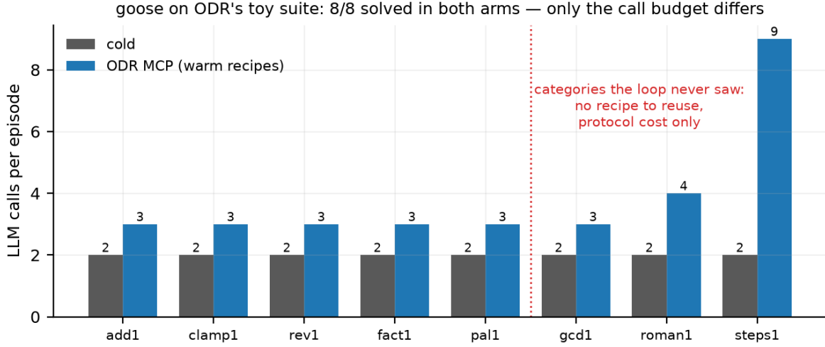
Figure 4: Warm-memory pull study on goose: per-episode LLM calls, cold vs. the ODR MCP server with promoted recipes attached. Solved fraction is 8/8 in both arms (not shown); the visible effect is the protocol cost, largest on categories the loop never saw.
