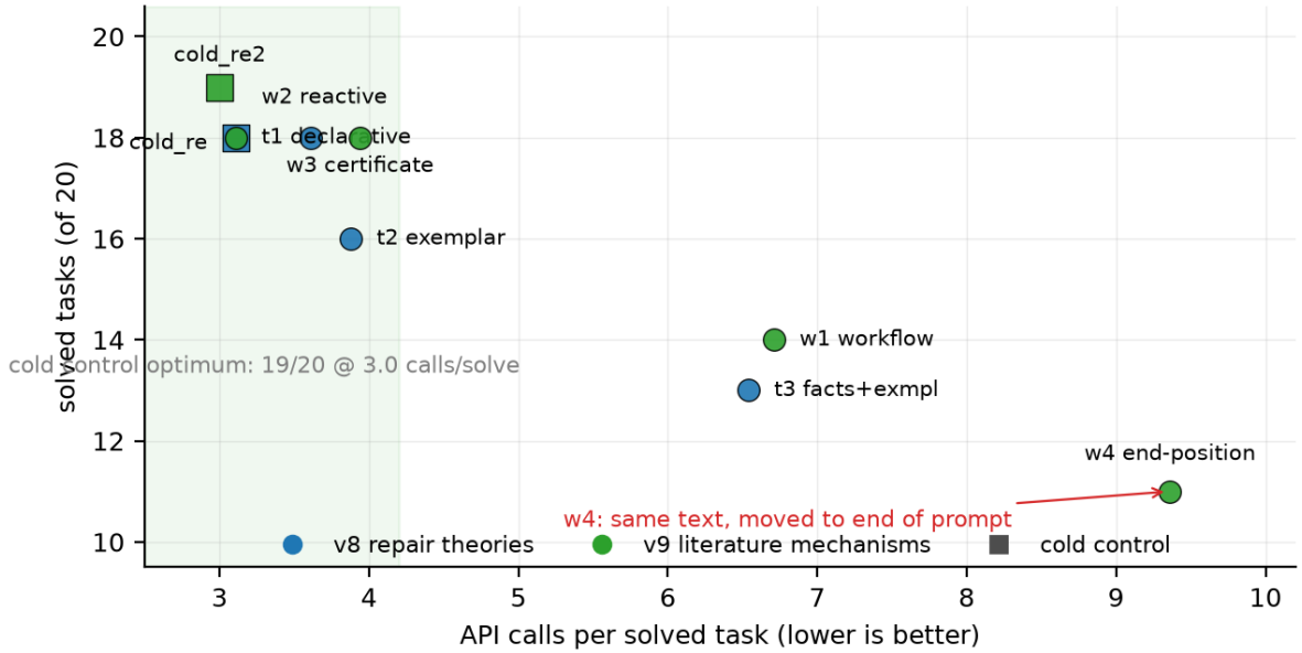
Figure 1: Injection-arm study on the live model (20 held-out tasks, greedy decode, one endpoint; v8 repair theories and v9 mechanisms each operationalize one published idea). Every arm is scored against the contemporaneous cold control run in the same sitting (squares). No arm beats cold; the gate rejects all of them. The end-position arm (w4) uses the identical text that is measured-safe mid-prompt (t1) — frame safety is position-dependent. Reactive-on-error injection (w2) pays zero prompt tax on clean episodes: the architecturally right channel, but with no benefit where cold is already optimal.
