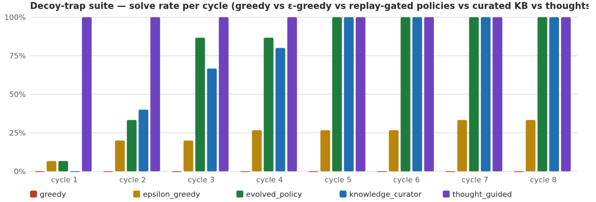
Figure 3: Per-cycle solve rate on the decoy-trap suite (mean over 3 seeds). Greedy never escapes the decoy; \varepsilon -greedy escapes by luck; replay-gated policies and the curated knowledge base saturate at 100% only after several cycles; thought-guided branching—the shipped library default—escapes every trap from the first cycle at the lowest total cost.
