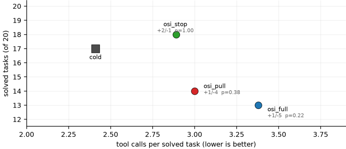
Figure 5: Cross-agent replication on goose: solved tasks vs. tool calls per solve, four arms, same tasks/scoring/model as the Hermes-side arms. Annotations give paired discordants against cold and exact McNemar p . The sentinel emitted no recurrence note on any episode (failures were one-off classes), yet pull-based access still cost solves — the tax is in the prompting, not in the notes.
