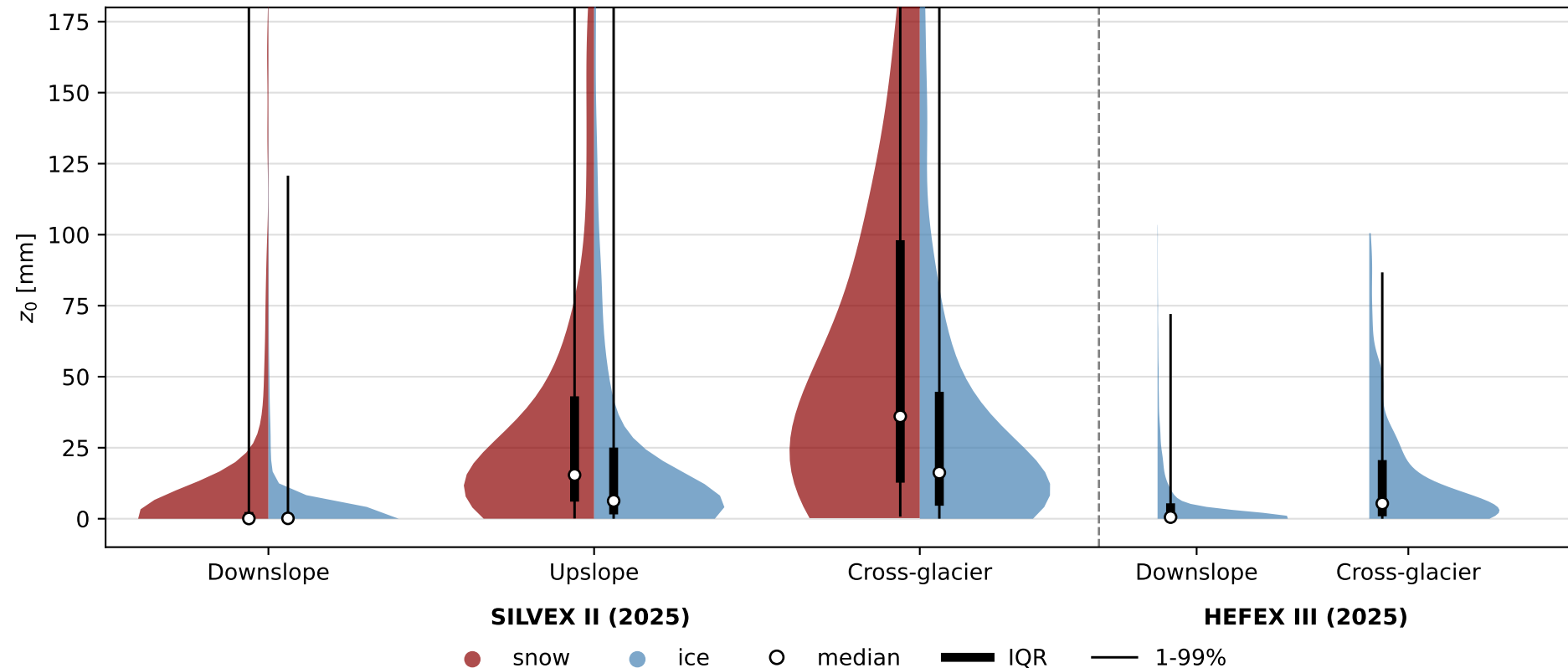
z_0 distributions from EC data by direction and surface type
