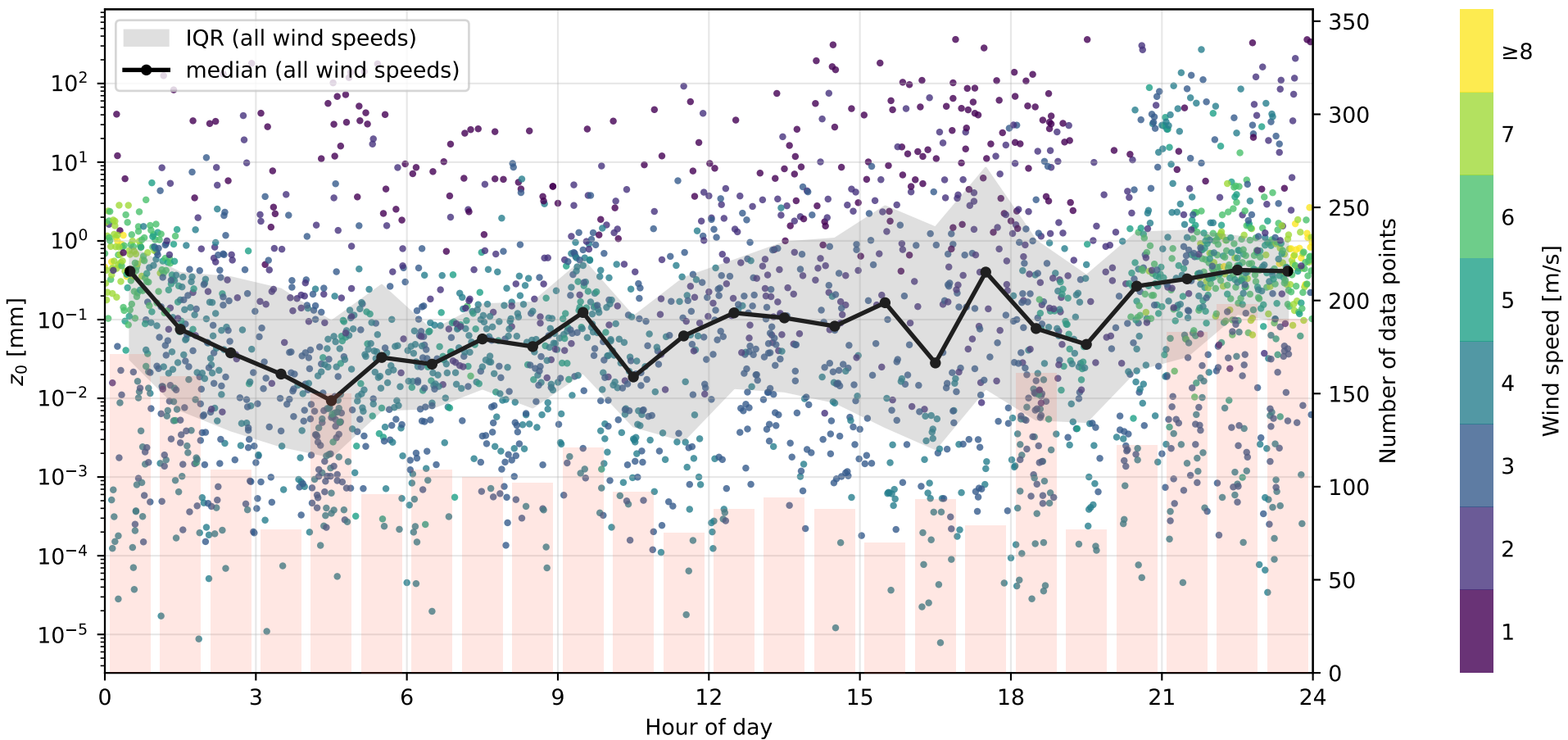
Diurnal pattern of z_0 (downslope, ice only)
