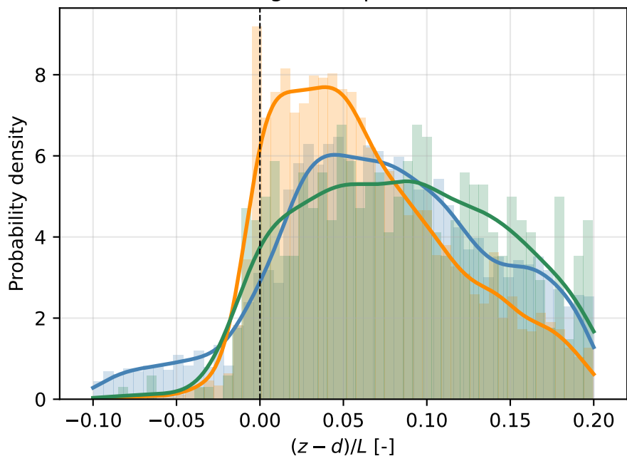
(z - d)/L by wind direction regime (histogram + plain KDE)
