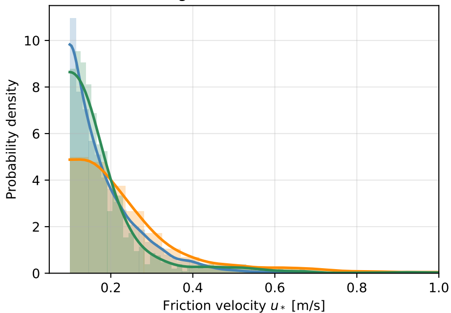
Friction velocity by wind direction regime (histogram + reflected KDE)
