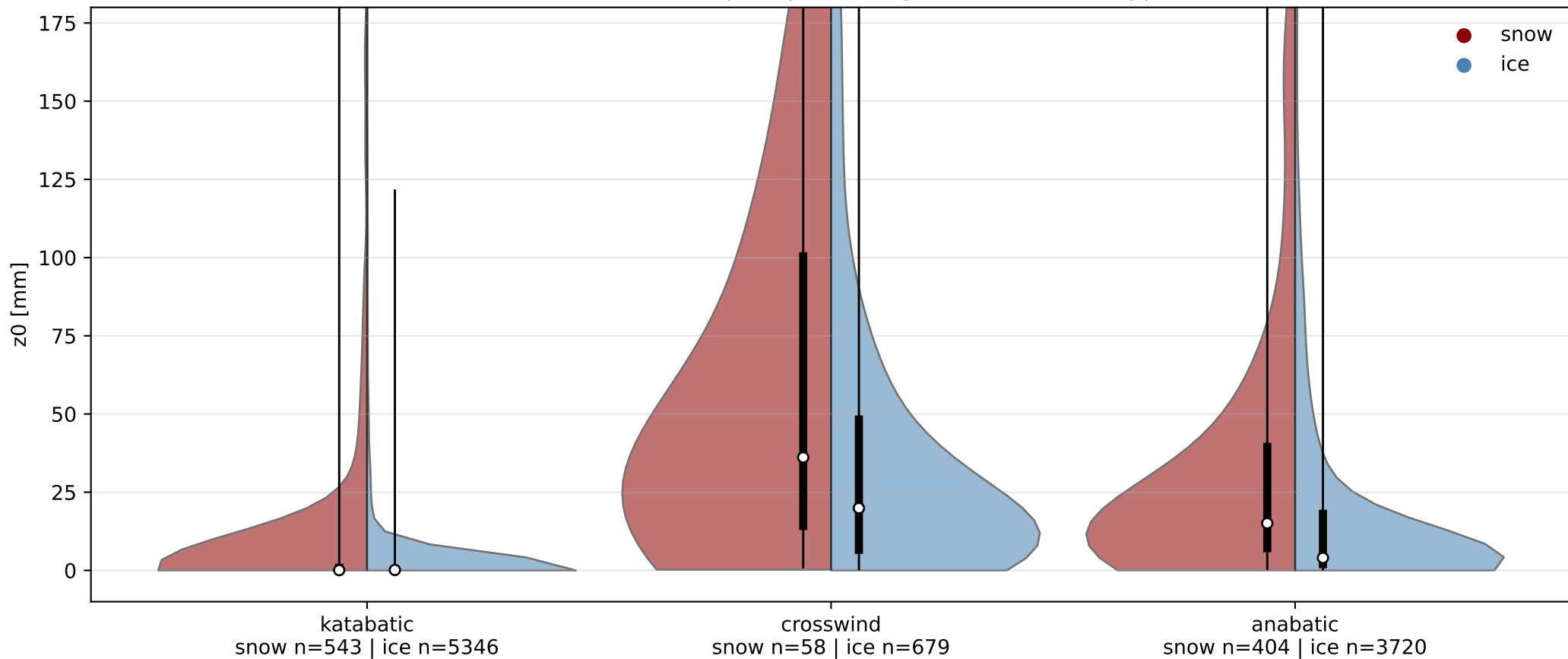
SILVEX II: z_0 (1 m) split by wind regime and surface type
