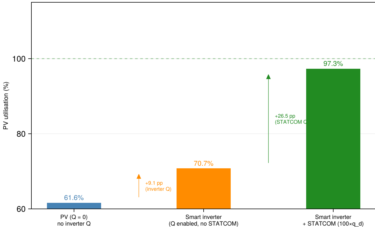
HC decomposition: inverter Q vs STATCOM Q contributions
