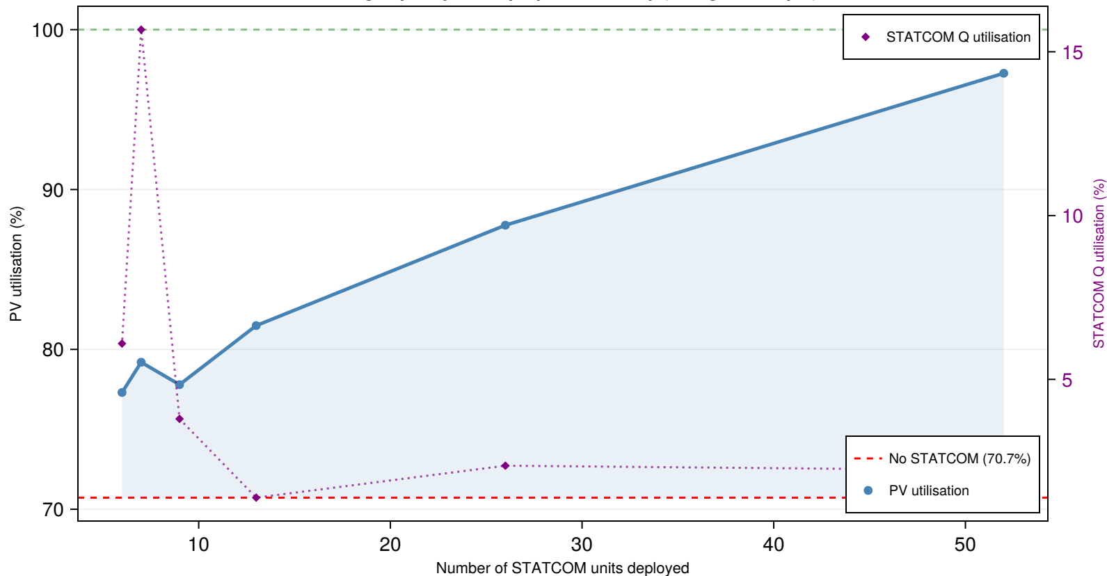
Hosting capacity vs. deployment density (rating = 100 \times q_d )
