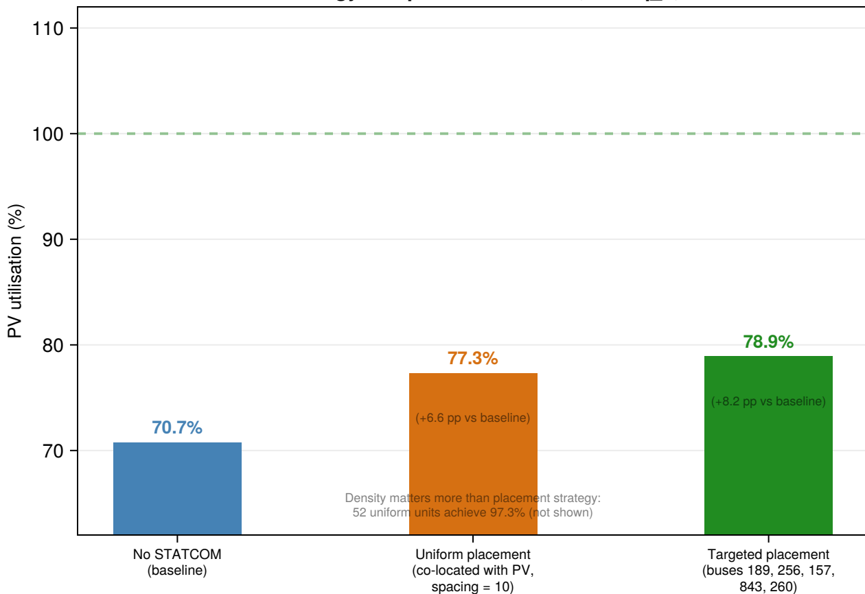
Placement strategy comparison — 5 units, 100×q_d, 5× stress
