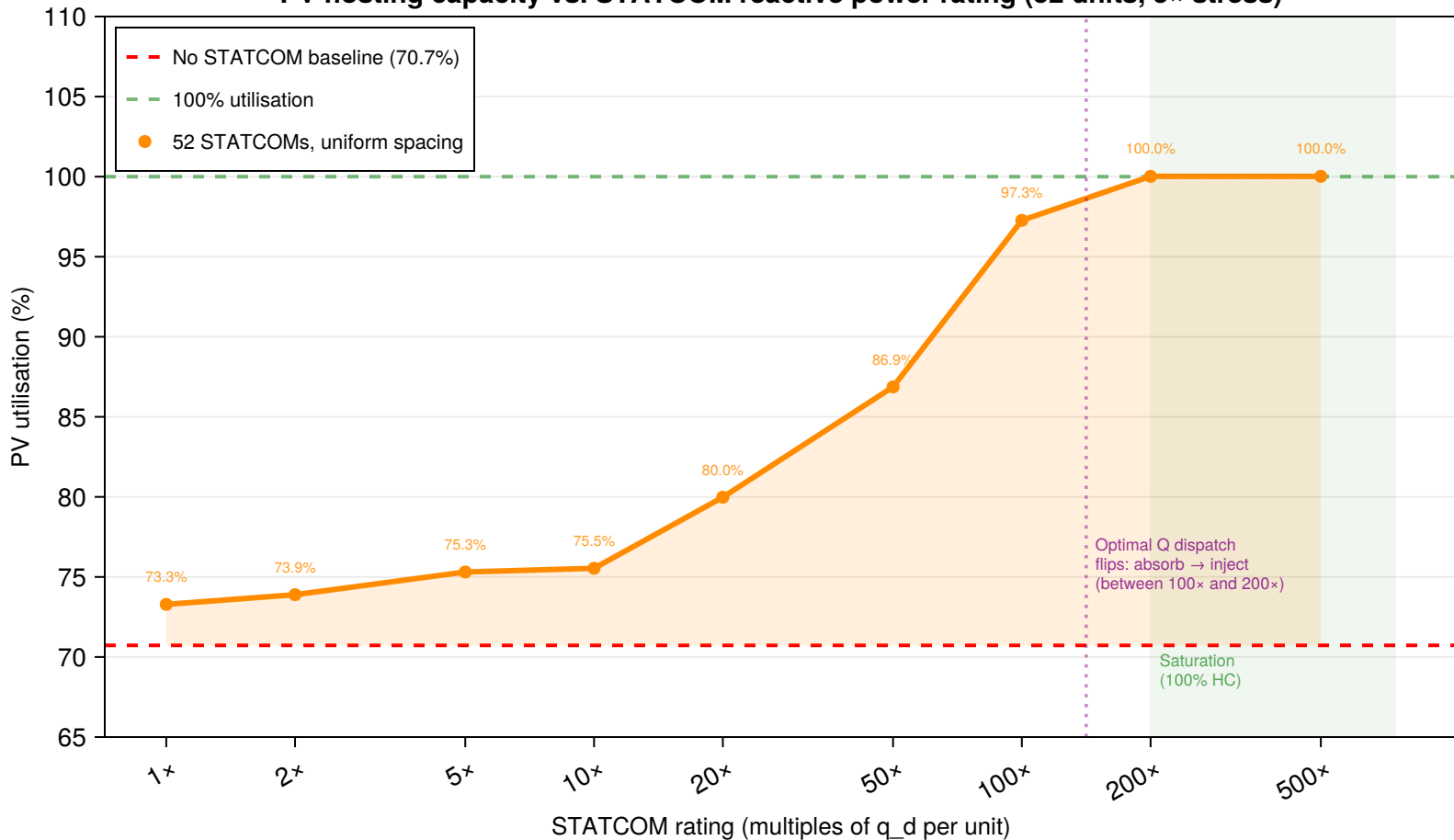
PV hosting capacity vs. STATCOM reactive power rating (52 units, 5× stress)
