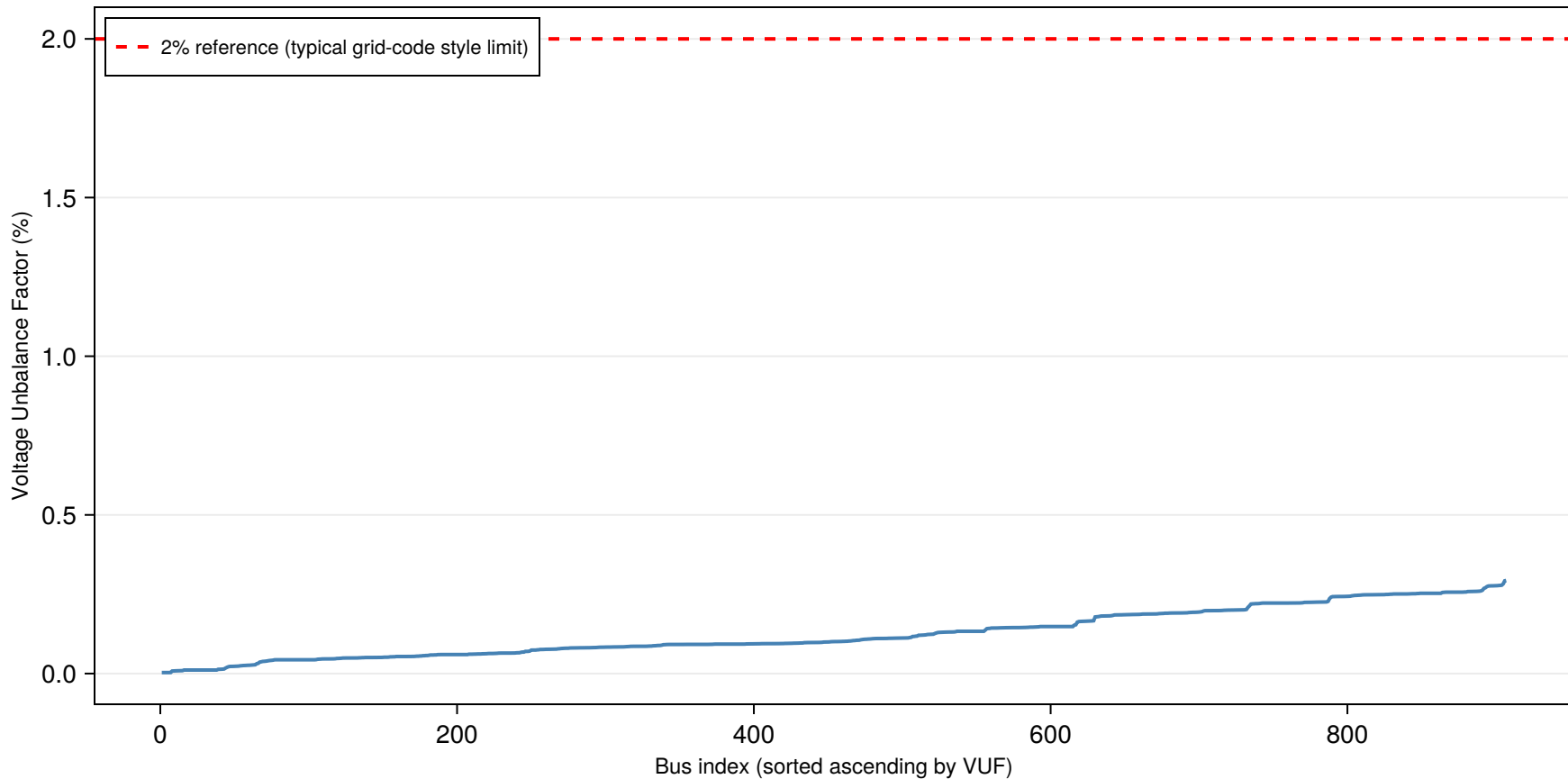
VUF at every bus -- natural network, no PV/STATCOM
