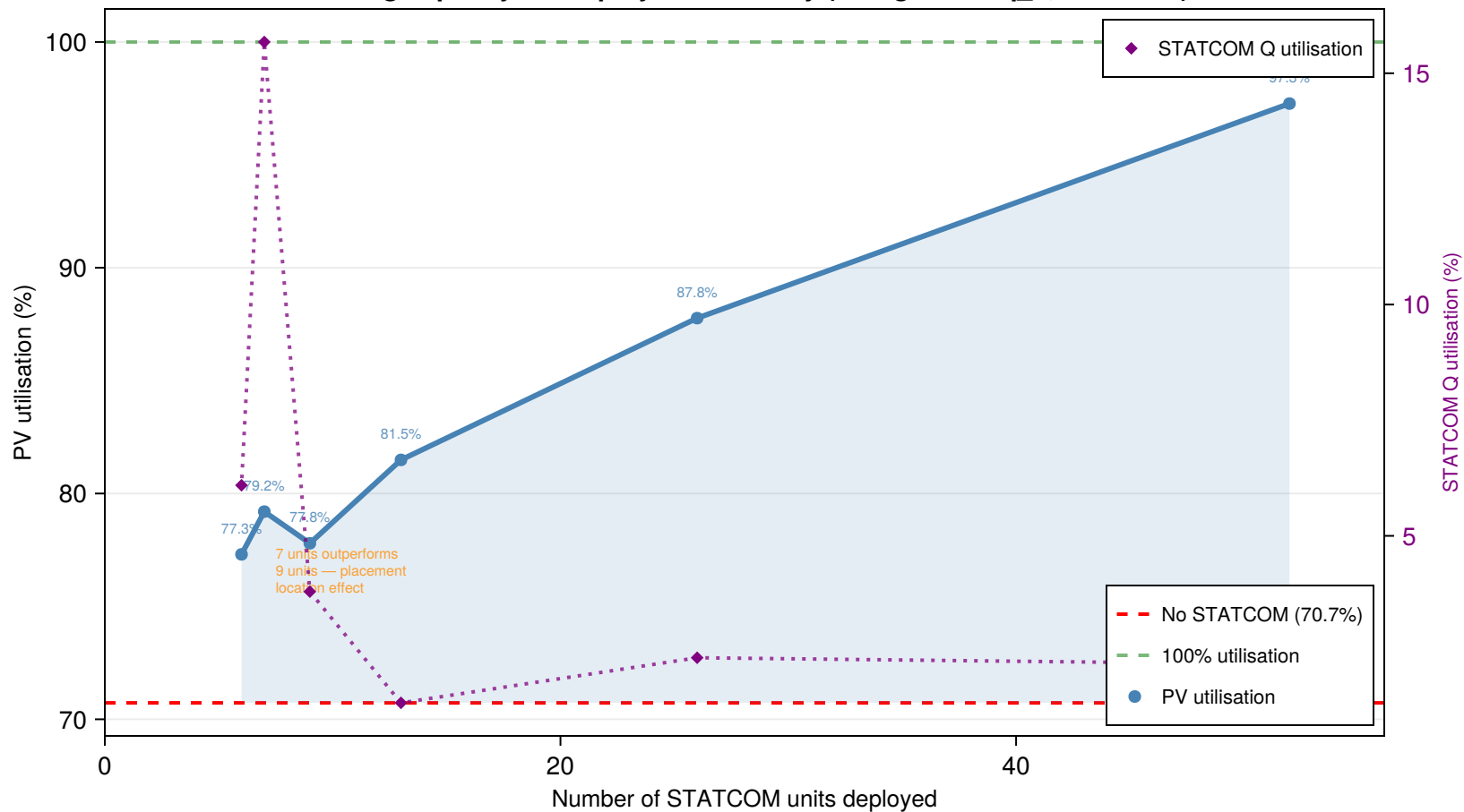
Hosting capacity vs. deployment density (rating = 100 \times q_d , 5 \times stress)
