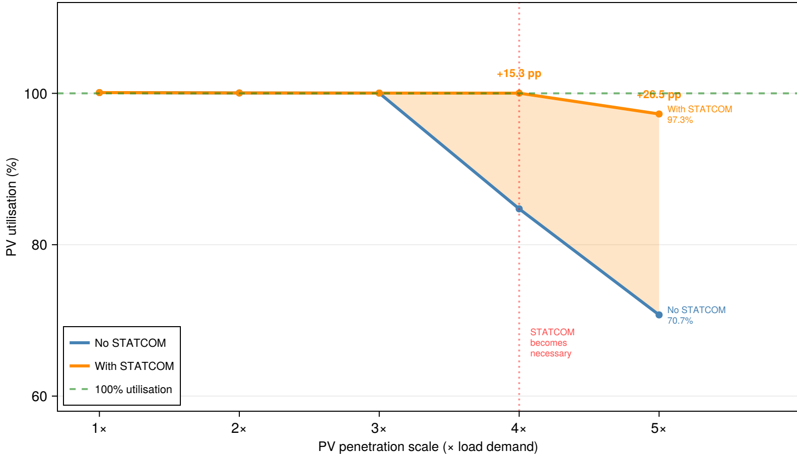
Hosting capacity: with and without STATCOM (100×q d , 52 units)
