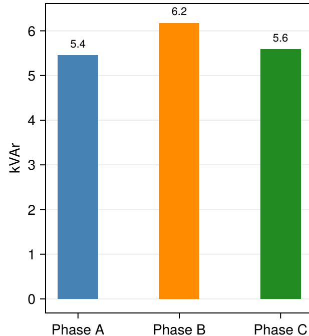
Total reactive demand per phase
