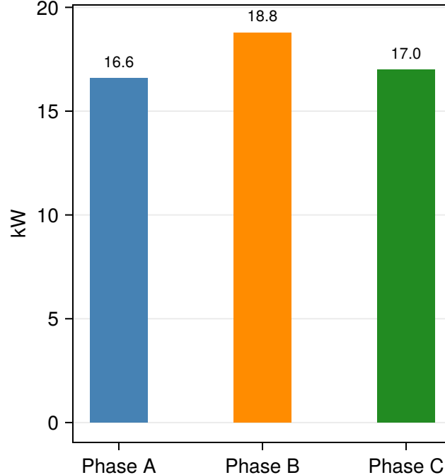
Total active demand per phase
