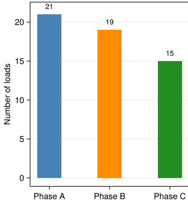
Load count per phase
