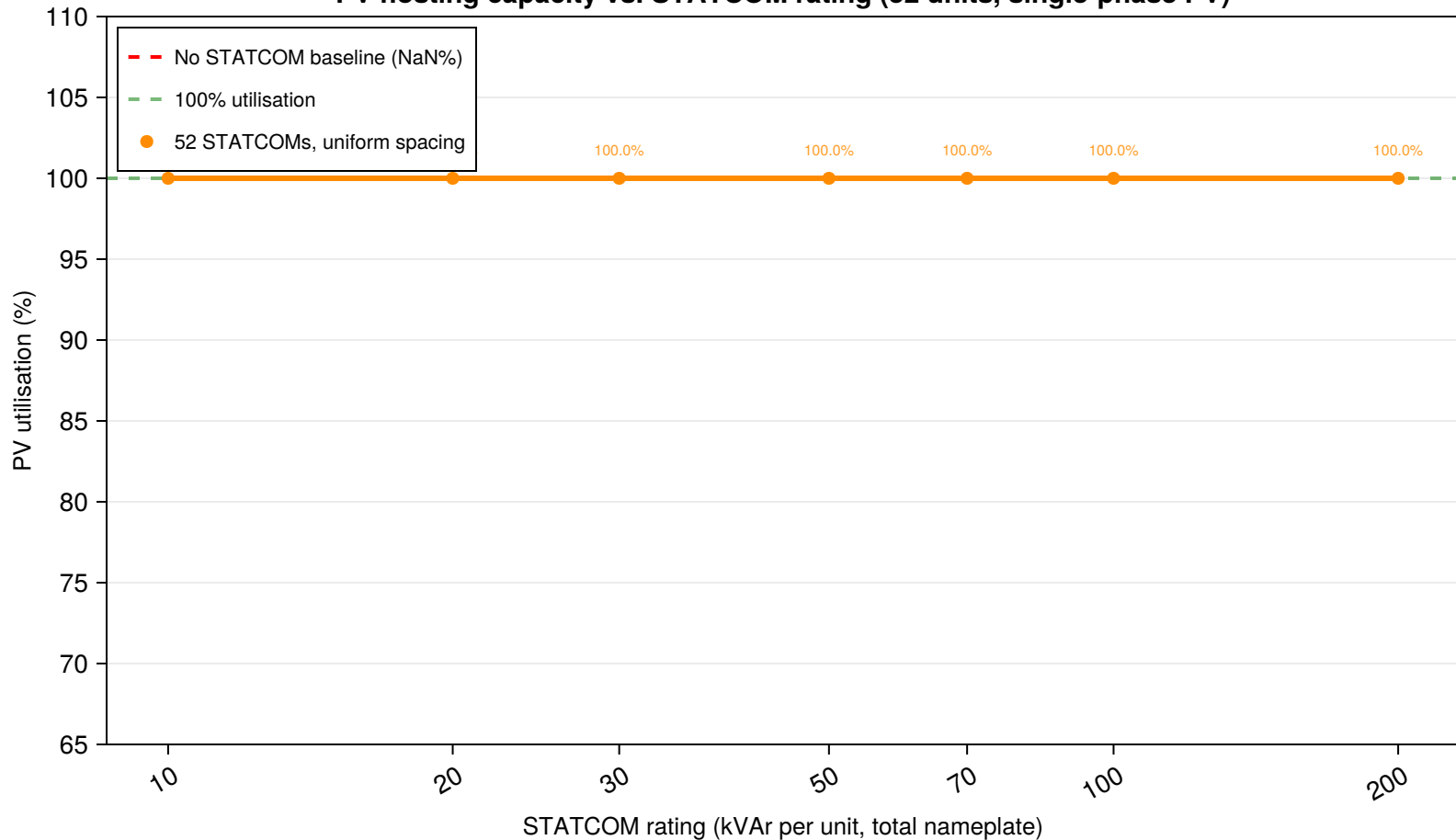
PV hosting capacity vs. STATCOM rating (52 units, single-phase PV)
