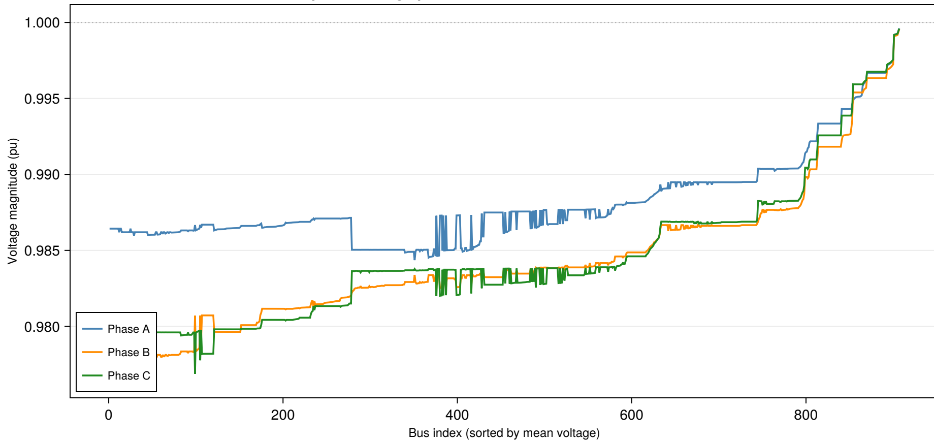
Per-phase voltage profile -- natural network, no PV/STATCOM
