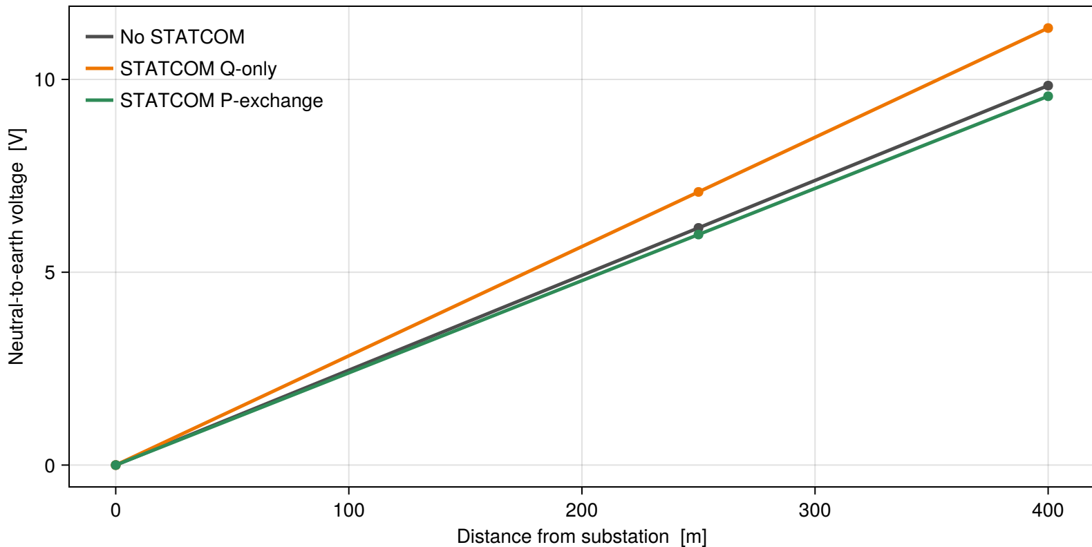
Neutral displacement at 16.0/1.5/0.5 kW split 10 \Omega MEN bond at the load bus; midbus unbonded
