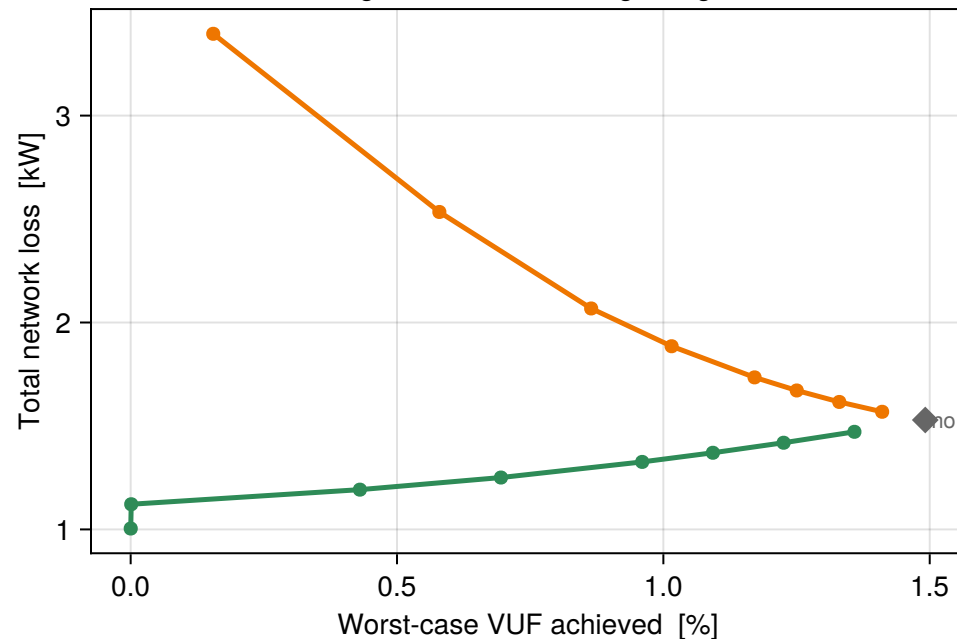
The trade-off right to left = increasing rating
