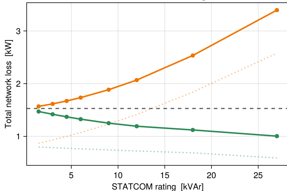
Loss vs converter rating
