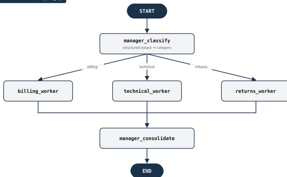
Figure 2.1b — The LangGraph implementation of this case study: manager_classify routes to exactly one worker node, which always returns through manager_consolidate .
