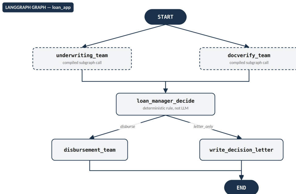
Figure 2.3b — The LangGraph implementation: underwriting_team and docverify_team are each a compiled subgraph called as one node from the top-level Loan Manager graph.
