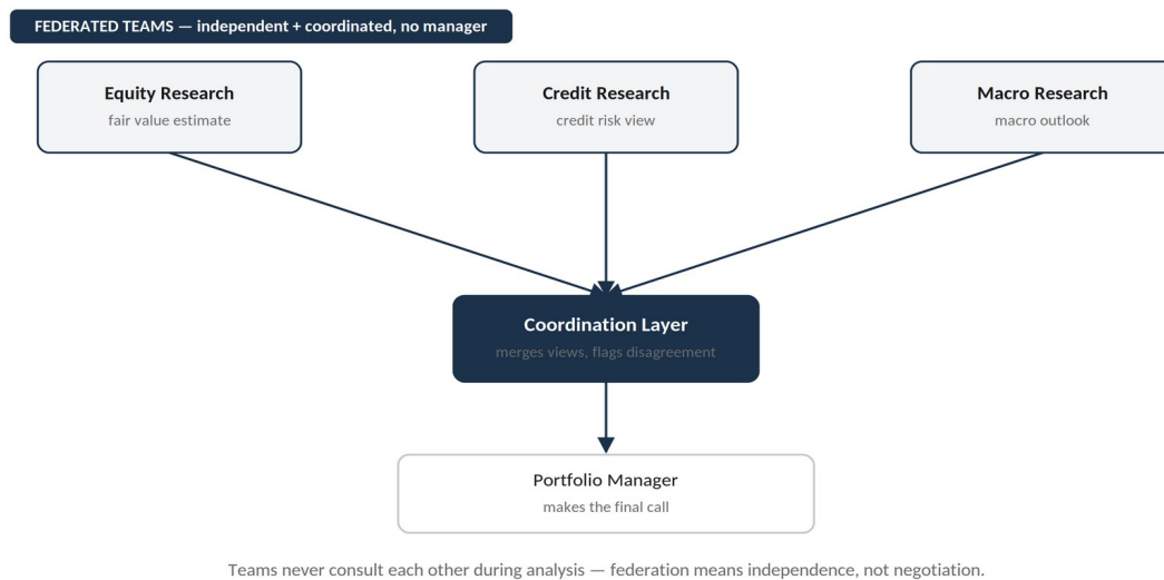
Figure 3.3 — Federated Teams: independent teams contribute in parallel; a coordinator merges views and flags disagreement.
