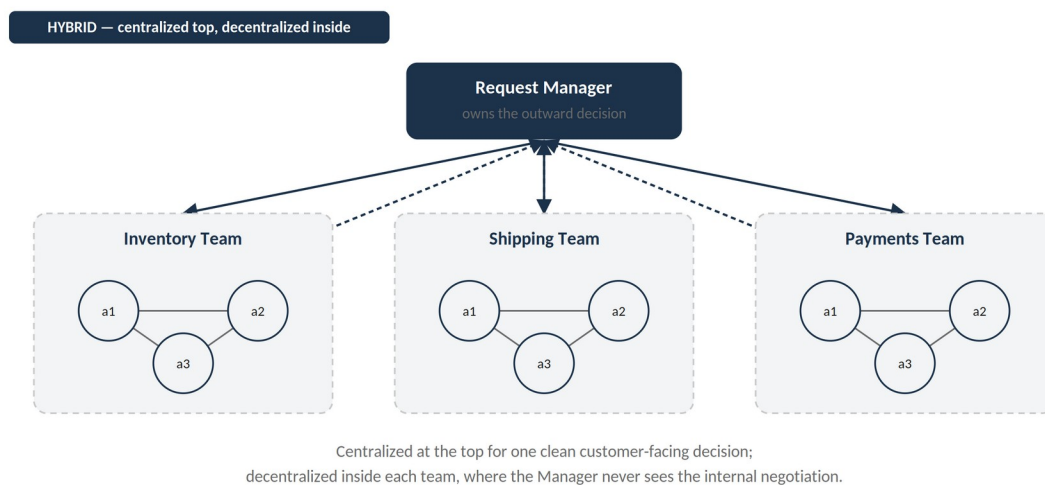
Figure 2.3 — Hybrid architecture: one central owner at the top, decentralized teams underneath.
