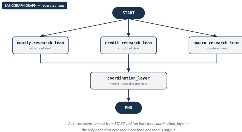
Figure 3.3b — The LangGraph implementation: three teams fan out from START and fan back into coordination_layer — the only node that sees more than one team's output.
