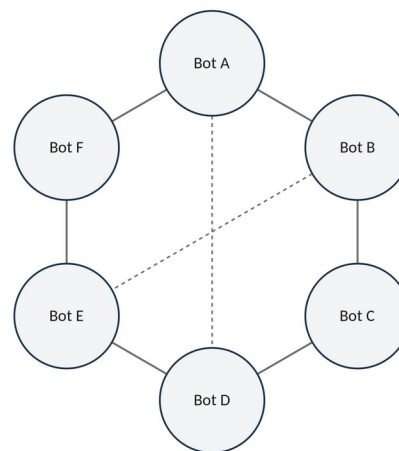
Figure 2.2 — Decentralized architecture: no central node; every bot senses and acts locally.
