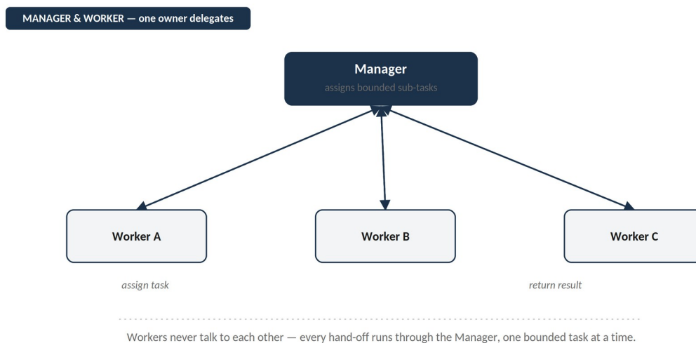
Figure 3.1 — Manager and Worker: bounded request and response, no Worker-to-Worker contact.
