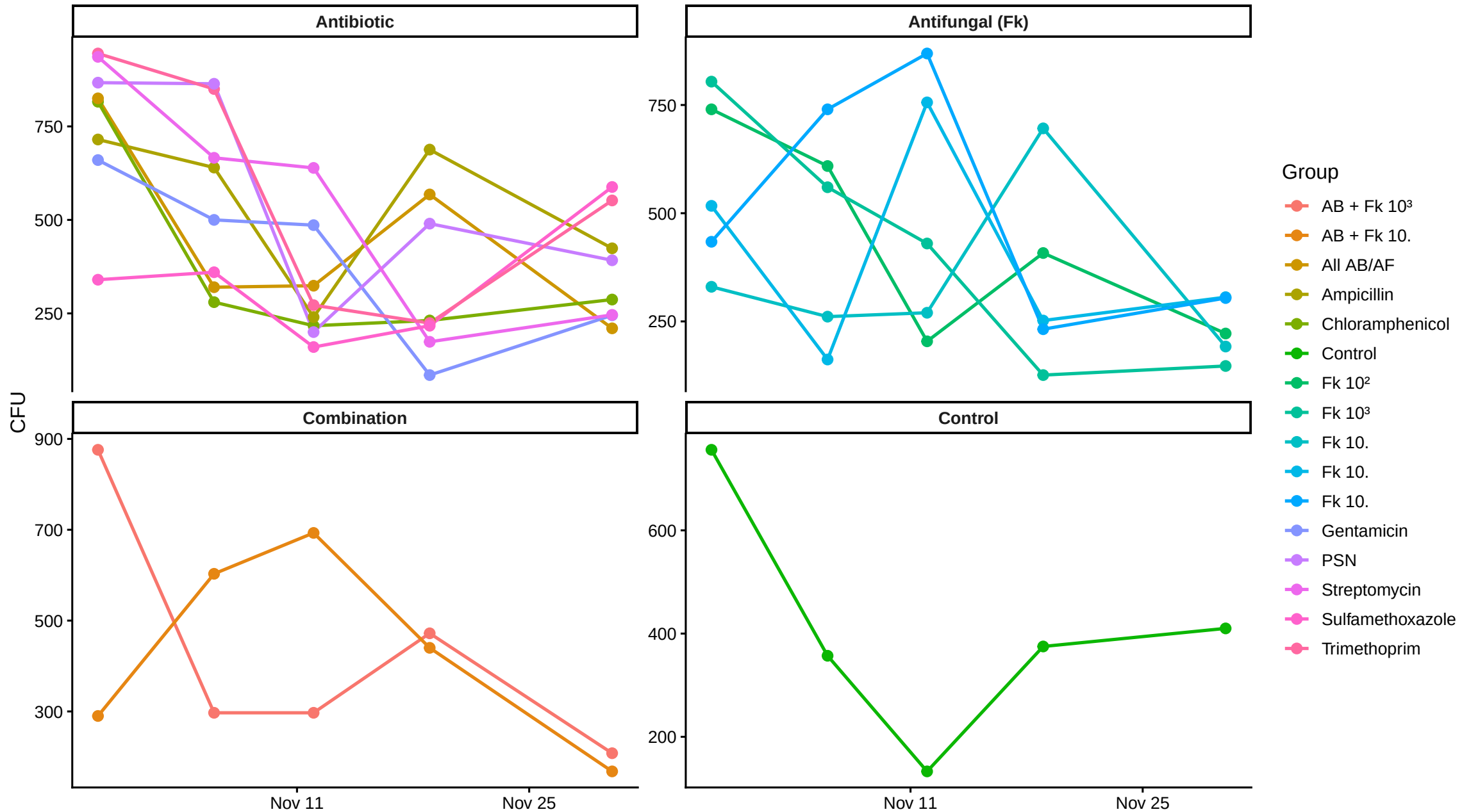
CFU over time – faceted by treatment category
